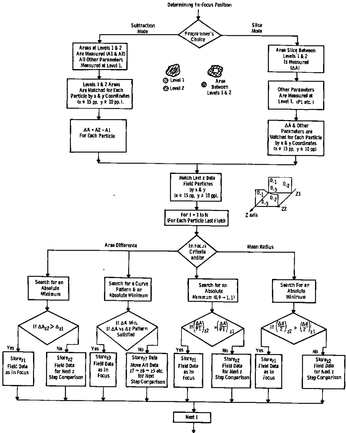
Figure 14. Flow chart of the focal detection algorithms.
