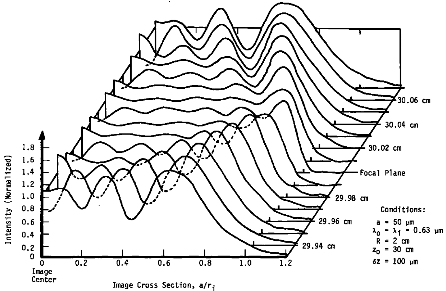
Figure 3. The intensity profiles of a particle image as a function of out-of-focus distance.
