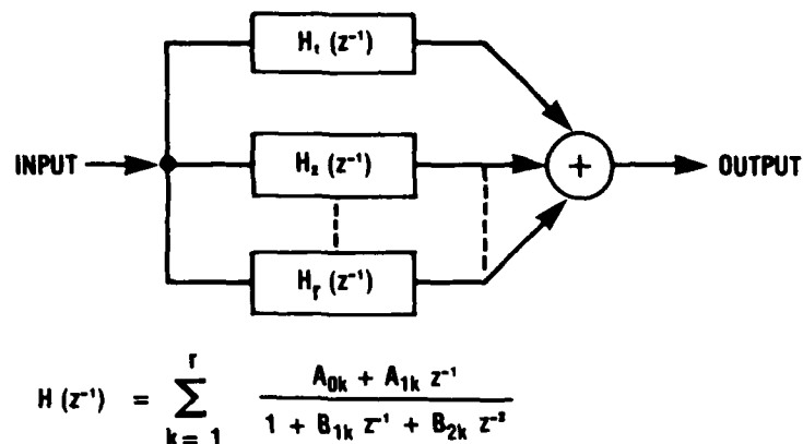
Figure 2. Recursive digital filter in parallel form.
