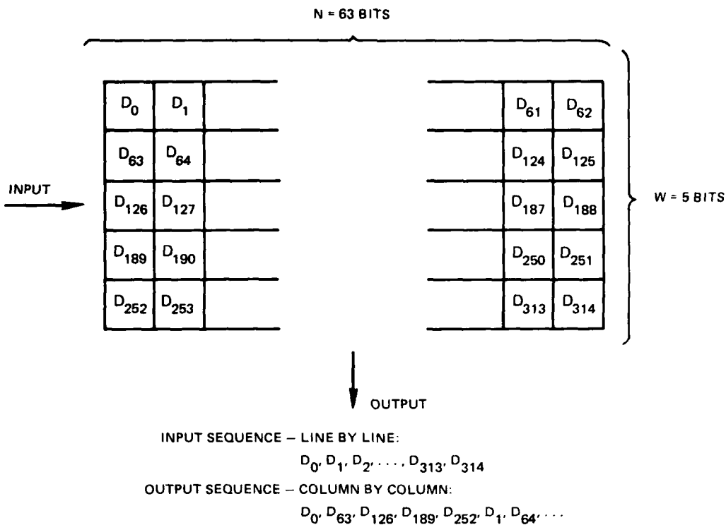
Figure D1. Interleaving buffer at the transmitter.
