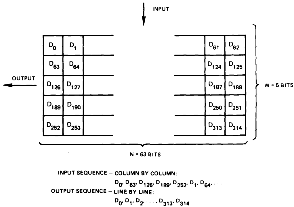
Figure D2. Interleaving buffer at the receiver.
