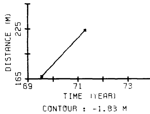
Figure 13. Distance from the base line to stated contours at MB 17.
