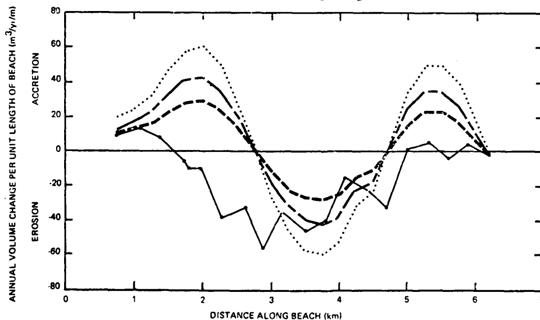
Figure 30. Comparison of measured and computed volumetric change along Wrightsville Beach.
