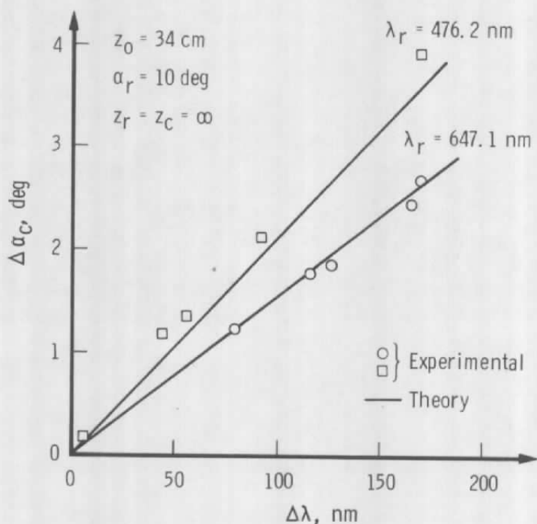
Figure 6. Angle change between recording and reconstruction versus wavelength change needed to obtain the best images.
