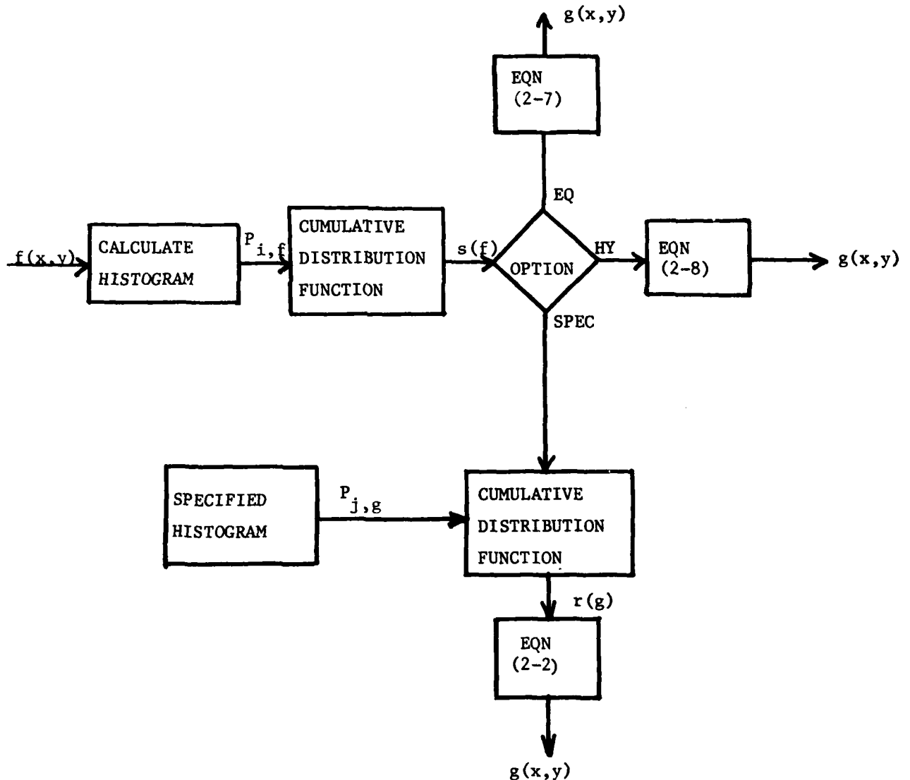
Figure 2.2 Histogram modification
