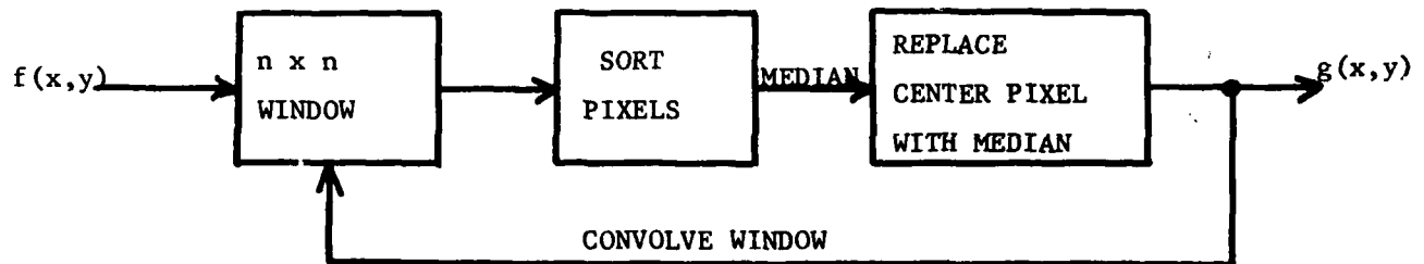
Figure 2.3 Median filter
