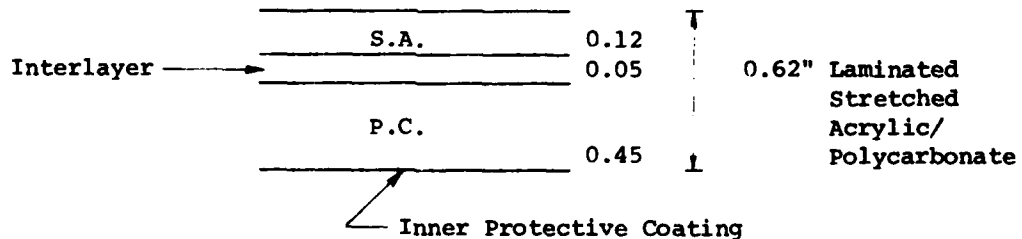
Reference AFWAL/FIEA Drawing No. 19260107-01
