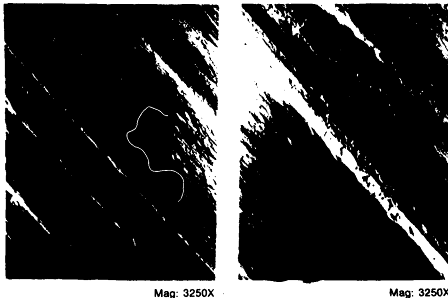
Figure 20. Unrubbed CRB-7 Ring Land Surface. Absence of Desirable "Moonscape" Textured Surface Was Apparent in Both Micrographs of an Unrubbed Ring Land Surface.
