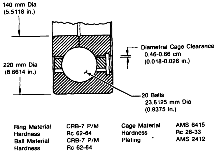
Figure 7 Design of The 140mm Bore Endurance Ball Bearing. This Bearing Has The Same Geometry as That of The Main Ball thrust Bearing in The TF33P-7, a Widely Used Transport Engine.
