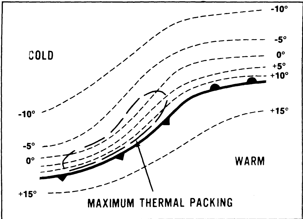
FIGURE 4.1. USING THE 850-MB ISOTHERM ANALYSIS TO LOCATE THE POLAR FRONT.
