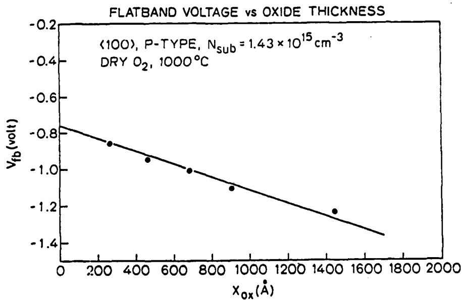
Fig. 8: Flatband voltage vs. oxide thickness for (100) P-type wafers oxidized at 1000^\circ\text{C} and fast pulled from \text{O}_2 ambient.
