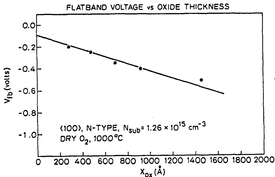
Fig. 7: Flatband voltage vs. oxide thickness for (100) N-type wafers oxidized at 1000^\circ\text{C} and fast pulled from \text{O}_2 ambient.
