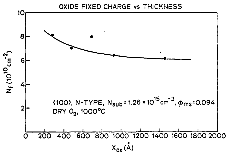
Fig. 12: Fixed oxide charge N_f vs. oxide thickness for (100) N-type wafers oxidized in dry O_2 at 1000^\circ\text{C} and fast pulled with no Ar anneal.
