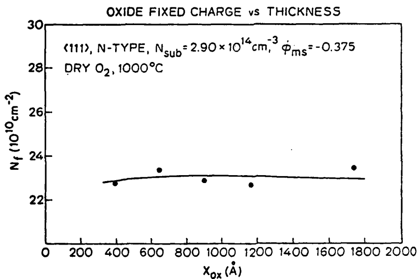
Fig. 13: Fixed oxide charge N_f vs. oxide thickness for (111) N-type wafers oxidized in dry O_2 at 1000^\circ\text{C} and fast pulled with no Ar anneal.
