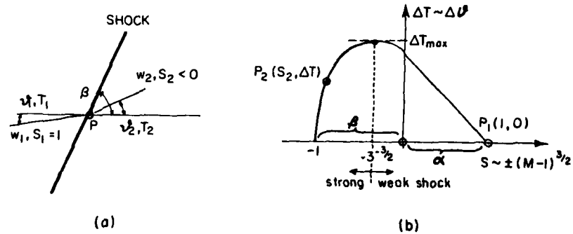
Fig. 6 Transonic Hodograph Variables and Shock Polar
