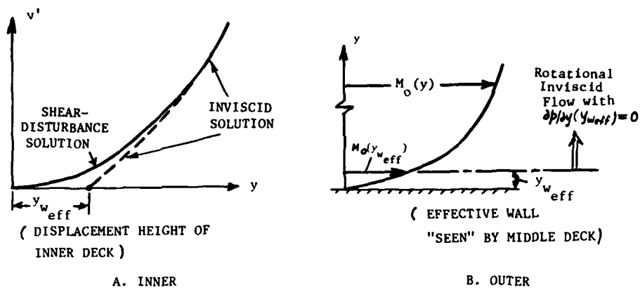
Fig. 4 Inner-Middle Deck Matching by the Effective Wall Concept
