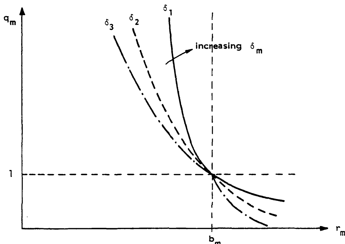
Figure 3.2 Modified Data Priority Function
