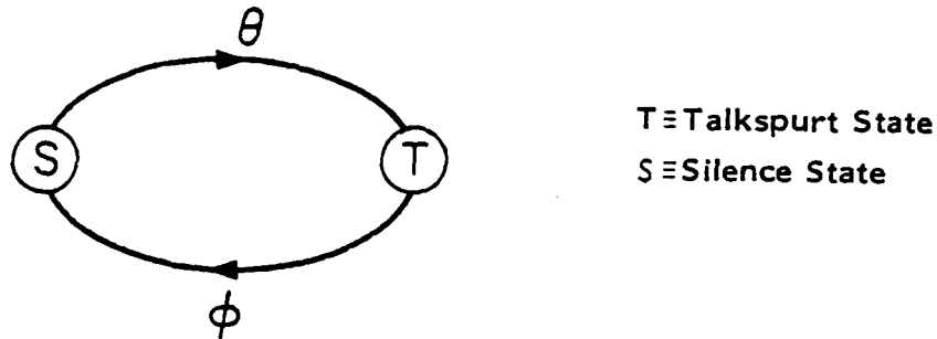
Figure 2.2 A Markov Chain Model of A Speaker
