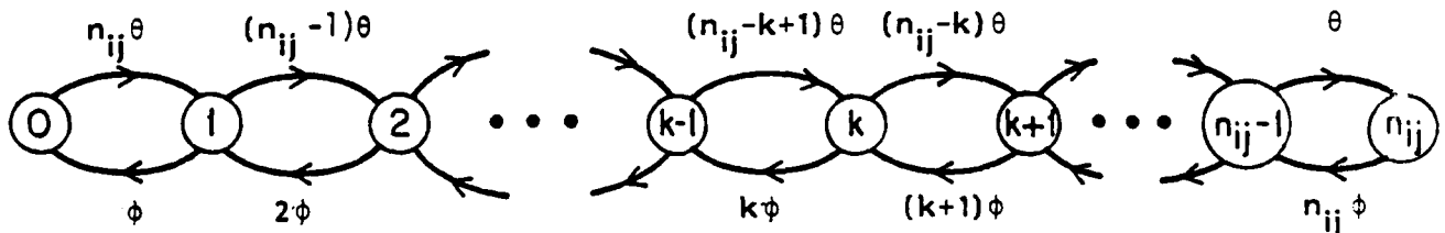
Figure 2.1 Speaker Activity Model for (i,j) Conversations
