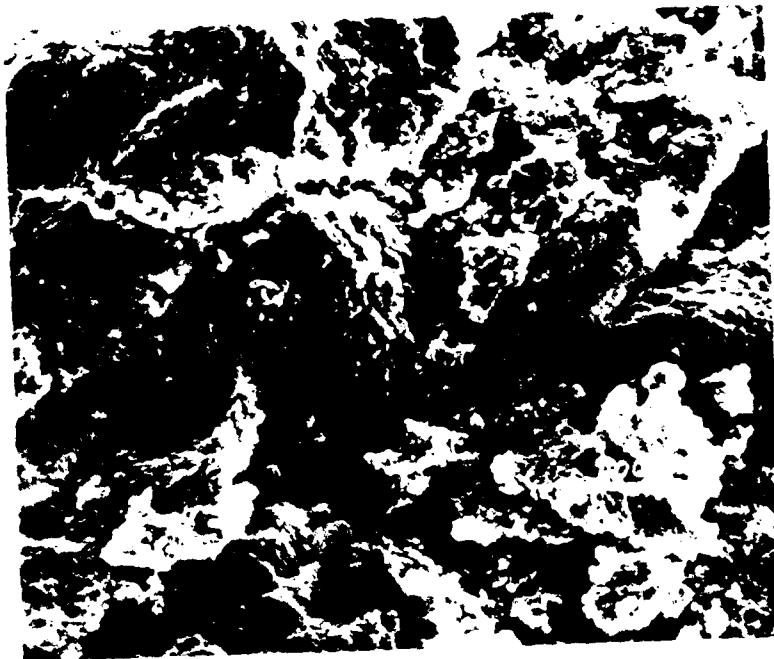
SEI micrograph showing broken surface of 7-day old mixture made with 1 part fume, 1 part CIL, and water to solids ratio about 1.2. Typical appearance at low magnification.
