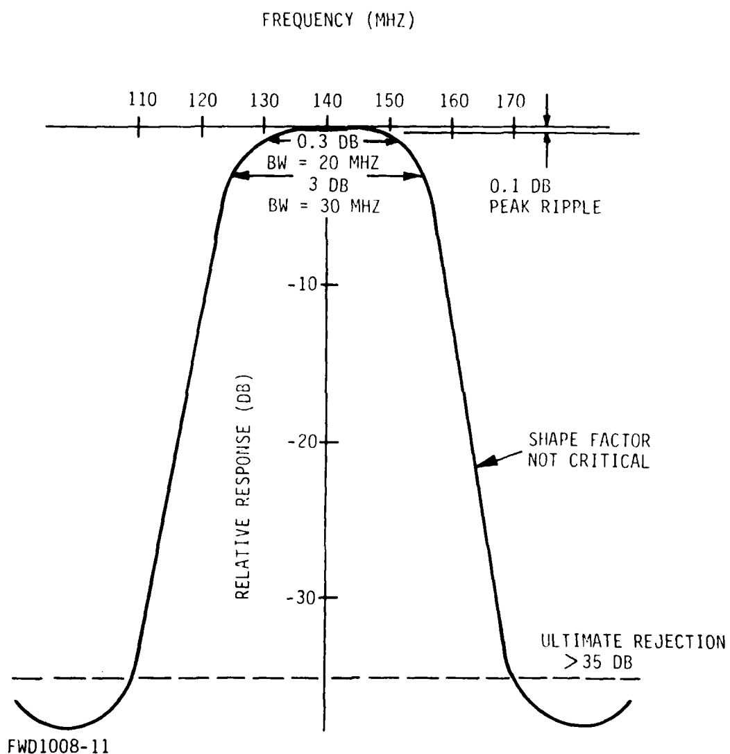
Figure 10. Desired Reponse of the Recirculating Integrator
