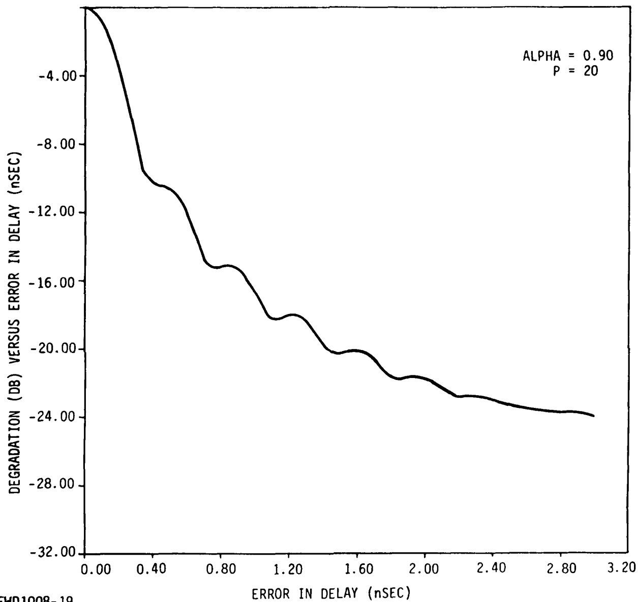
Figure 23. Degradation (dB) Versus Error in Delay (nSec)
