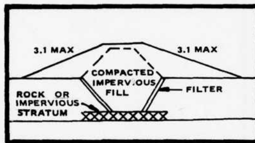
Figure 2-3A Levee with Impervious Core
