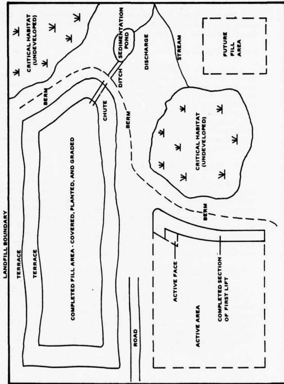
Figure 2-6. Selective Landfilling
