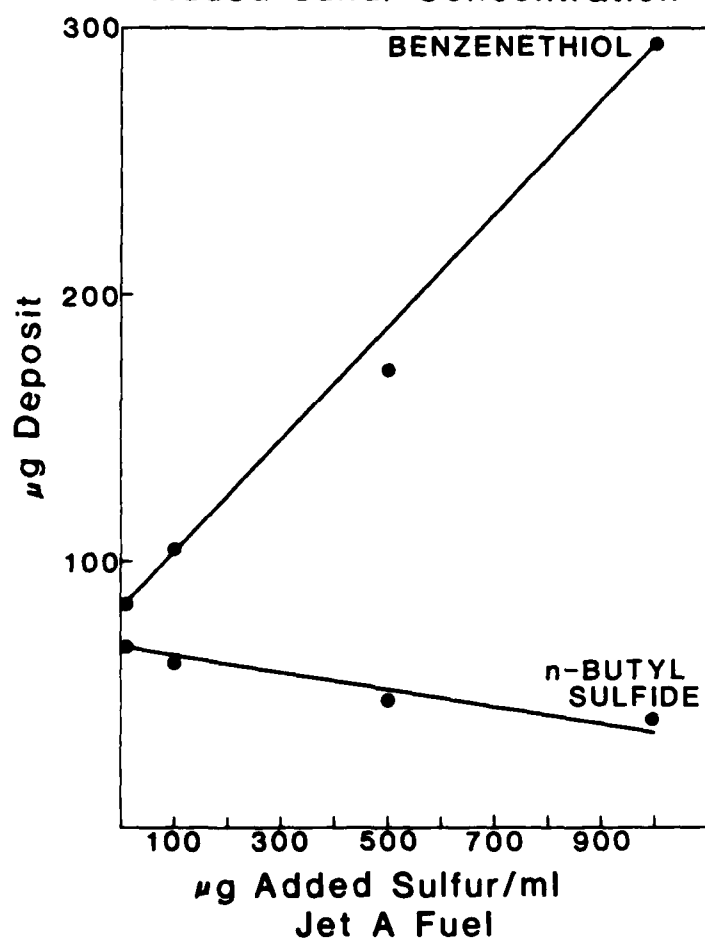
FIGURE VI Deposit Versus Added Sulfur Concentration
