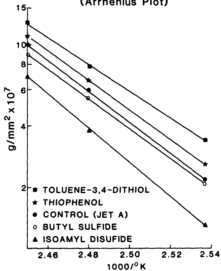
FIGURE VIII Temperature Dependence of Sulfur Compound Effects (Arrhenius Plot)
