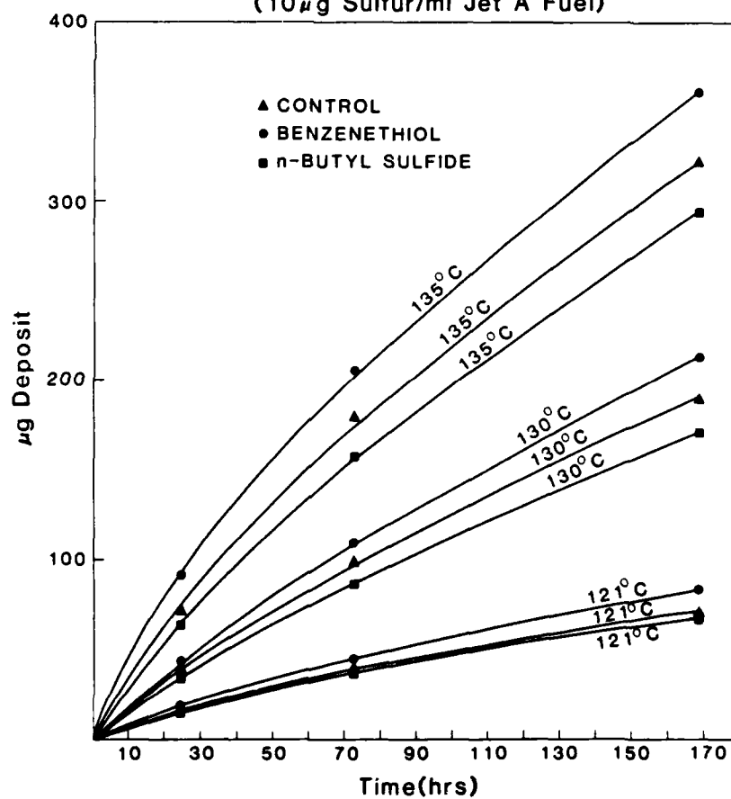
FIGURE VII Effect of Temperature upon Deposit Weight (10 \mu\text{g} Sulfur/ml Jet A Fuel)
