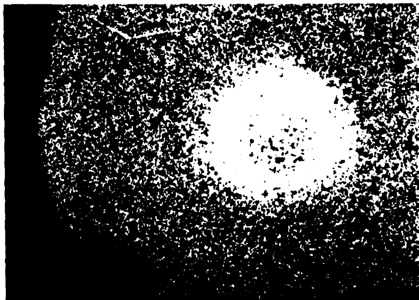
FIGURE X: Jet A Fuel Spiked with n-Butyl sulfide and Stored at 121°C, 168 hours
