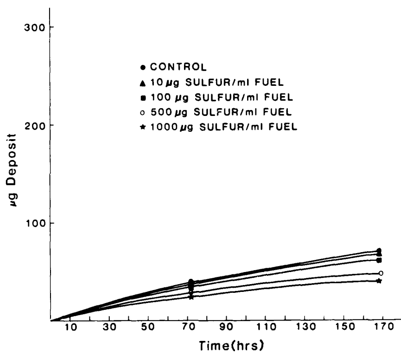
FIGURE V Effect of Added Sulfur Concentration on Deposition Rate (n-Butyl Sulfide, 121°C)
