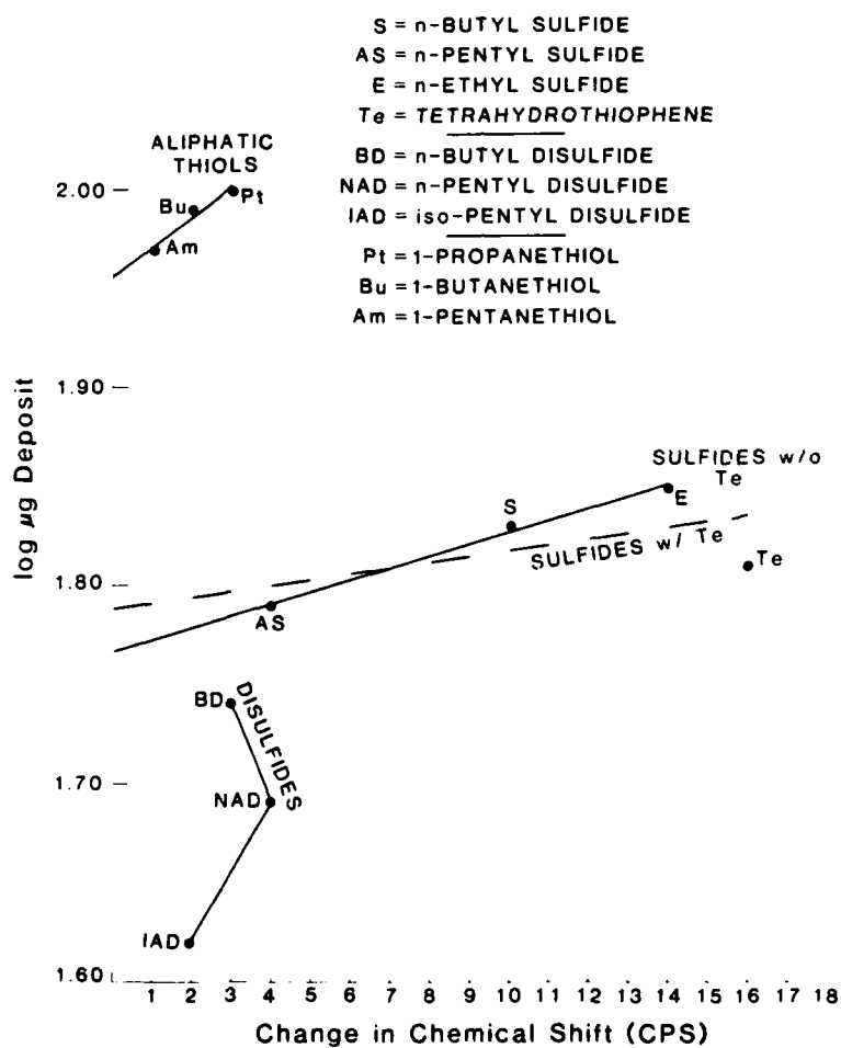
FIGURE XXIII Jet A Deposit Weight (121°C) and PNMR Chemical Shift Change
