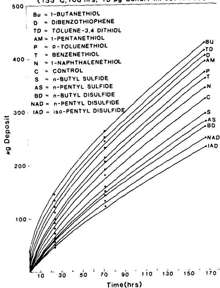
FIGURE III Effect of Added Sulfur-Containing Compounds on Deposition Rate
