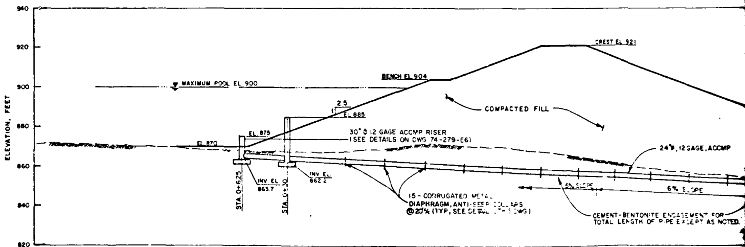
SECTION B-B - PROFILE ALONG Q DECANT SY
