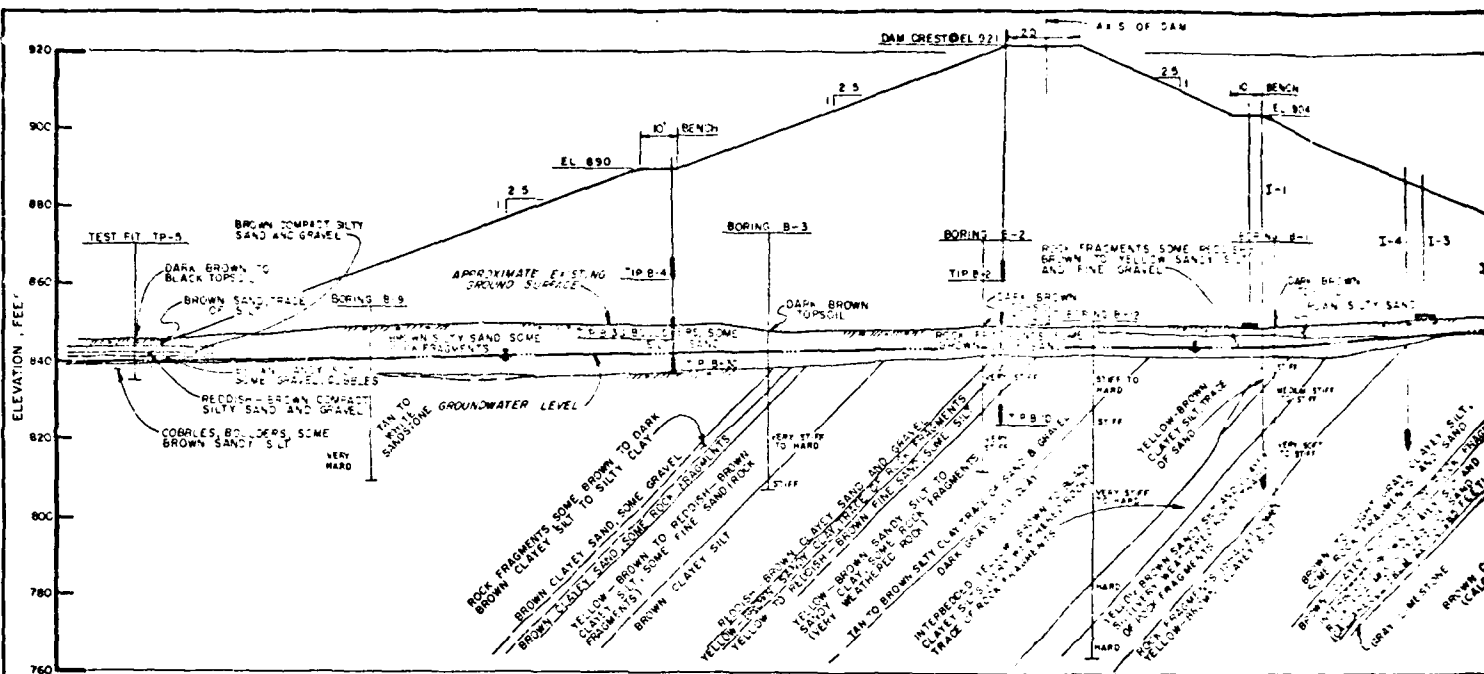
SECTION C-C
