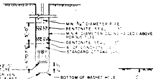
PIEZOMETER DETAILS
