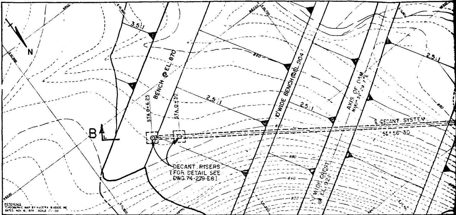
PLAN - DECANT SYSTEM
