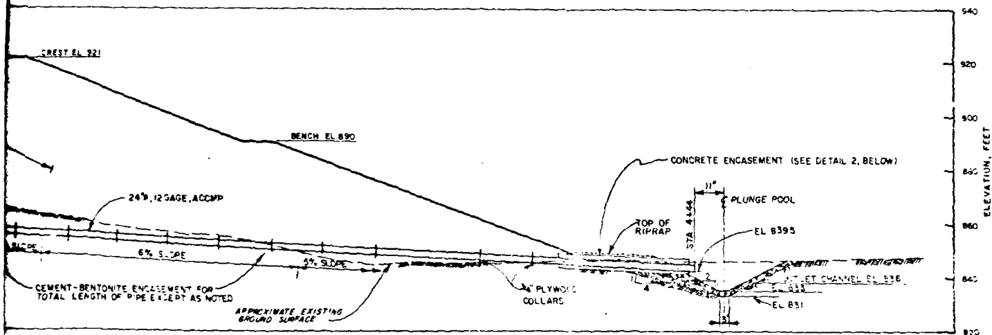
FILE ALONG C. DECANT SYSTEM
