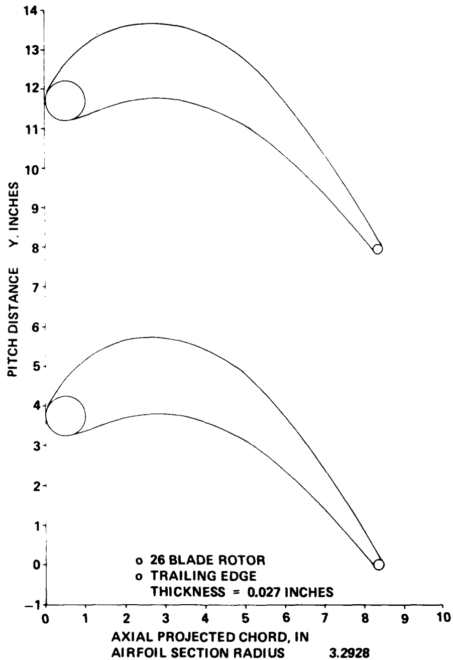
Figure 53 . EG Preliminary Rotor Hub Section.
