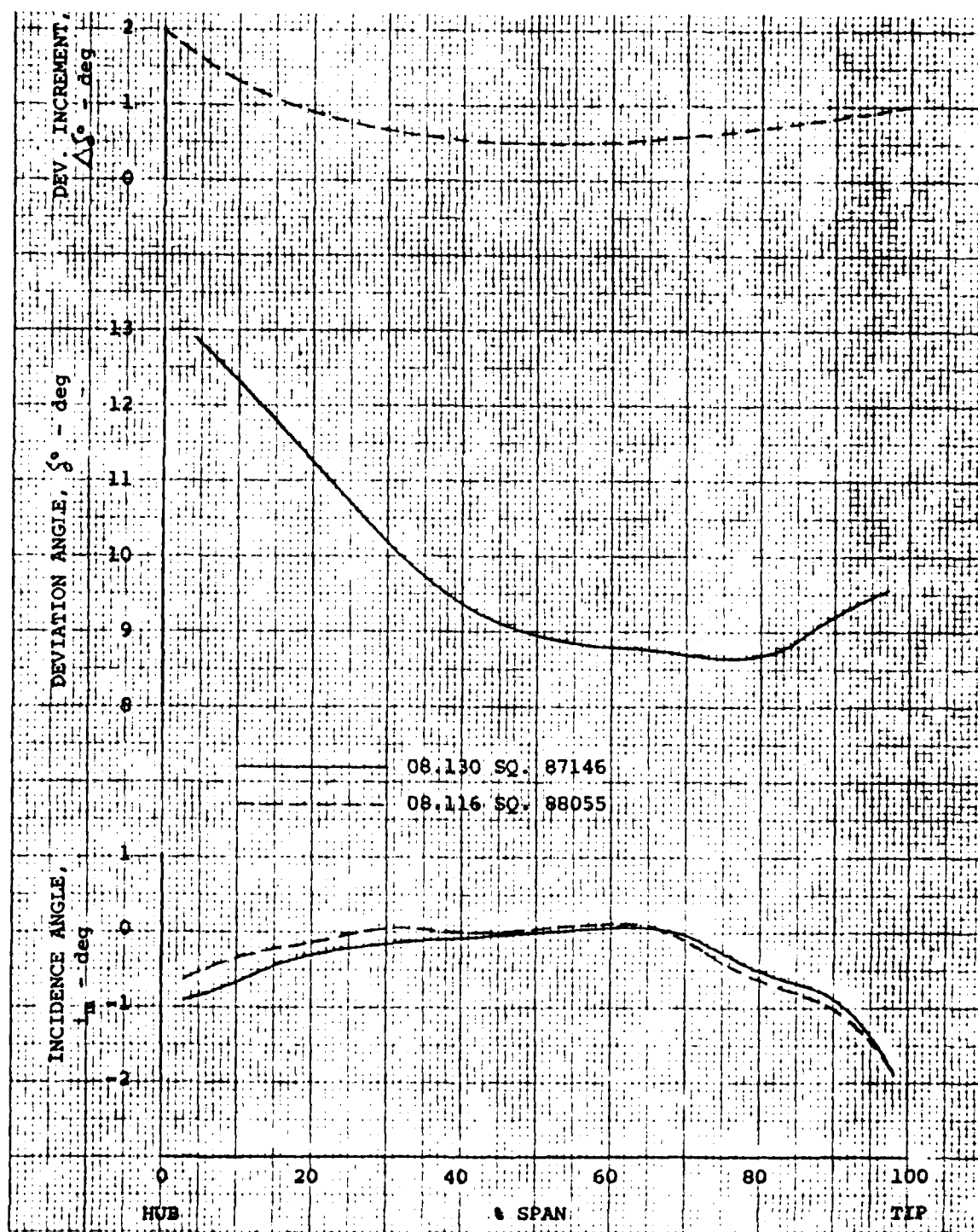
Figure 113. Expendable Gasifier Compressor Second Stage Rotor Incidence and Deviation. 27282
