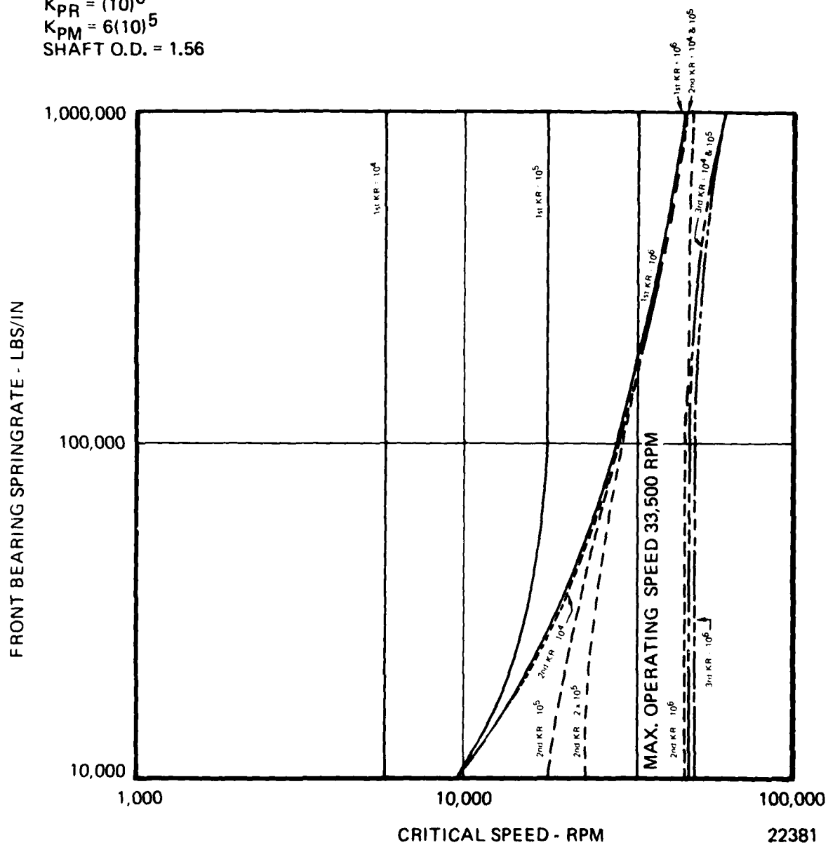
Figure 65 . Expendable Gasifier Critical Speeds.
