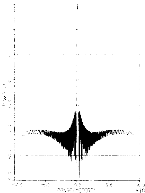
Fig. 2 — Response of a Hamming weighted pulse compression filter to a noise-free target signal
