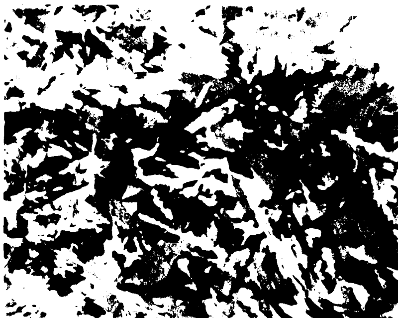
Figure 26. Showing structure 70mm from end of end quenched bar after ageing 3 hours 450°C. CROSSED POLARS
