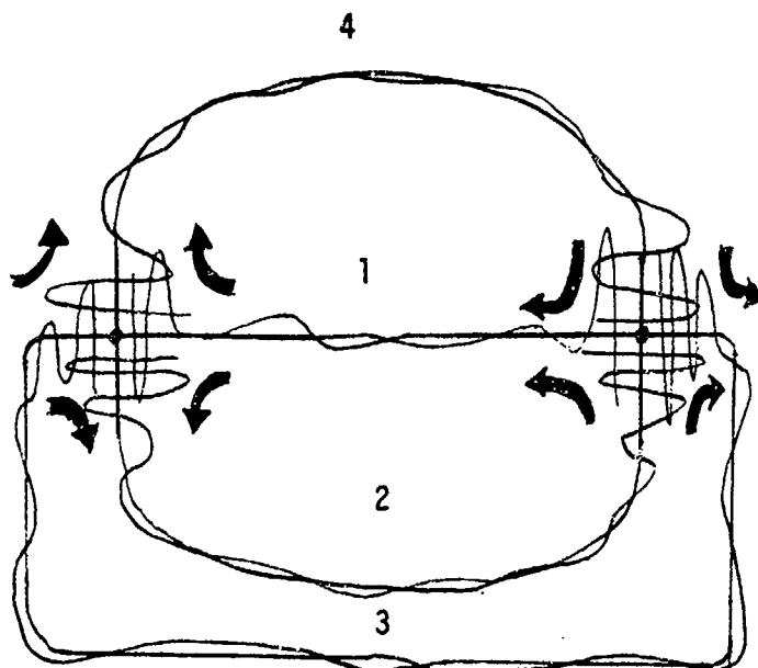
Figure 5. The homoclinic structure of the perturbed manifold W^S(0, \pm l, 0) , W^N(0, \pm l, 0) on the sphere.
