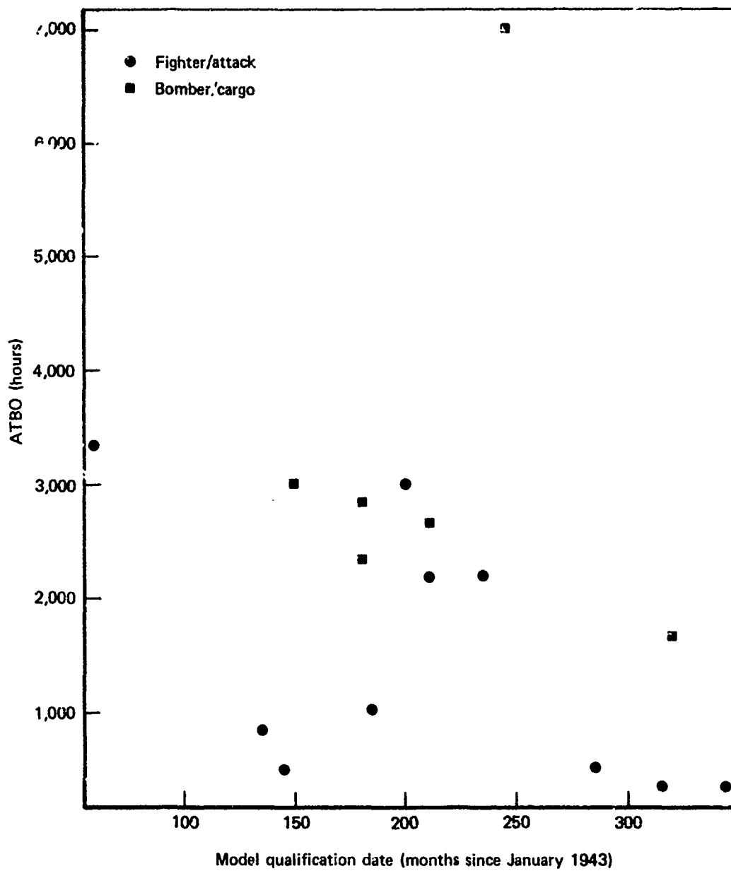
Fig. E.18—Variation of ATBO with model qualification date
