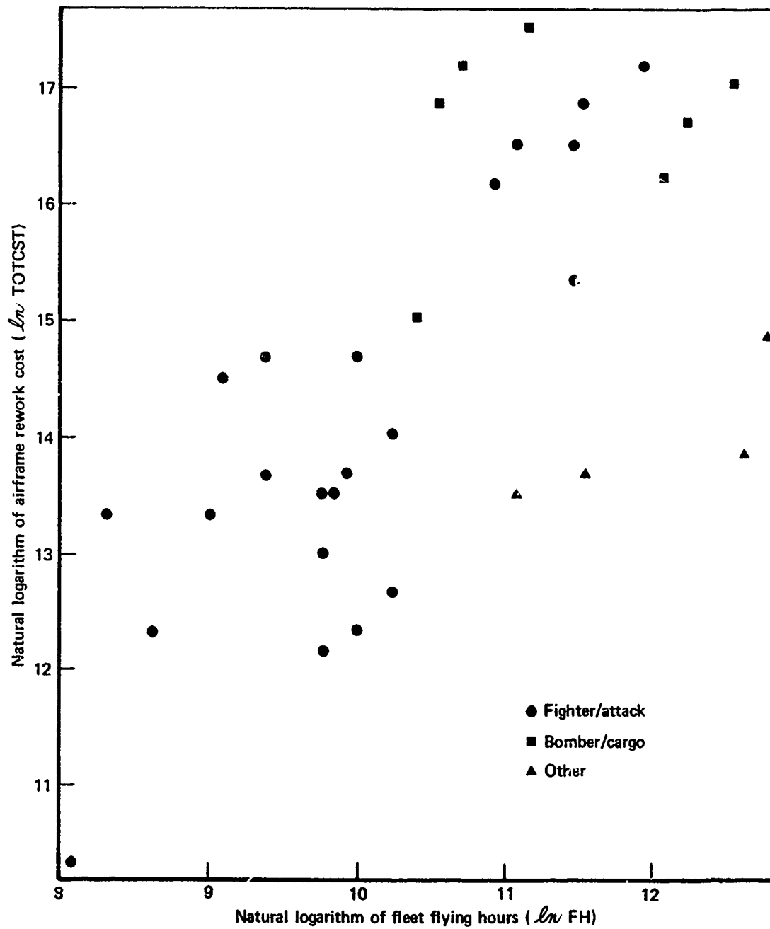
Fig. F.1—Variation of total airframe rework cost with fleet flying hours
