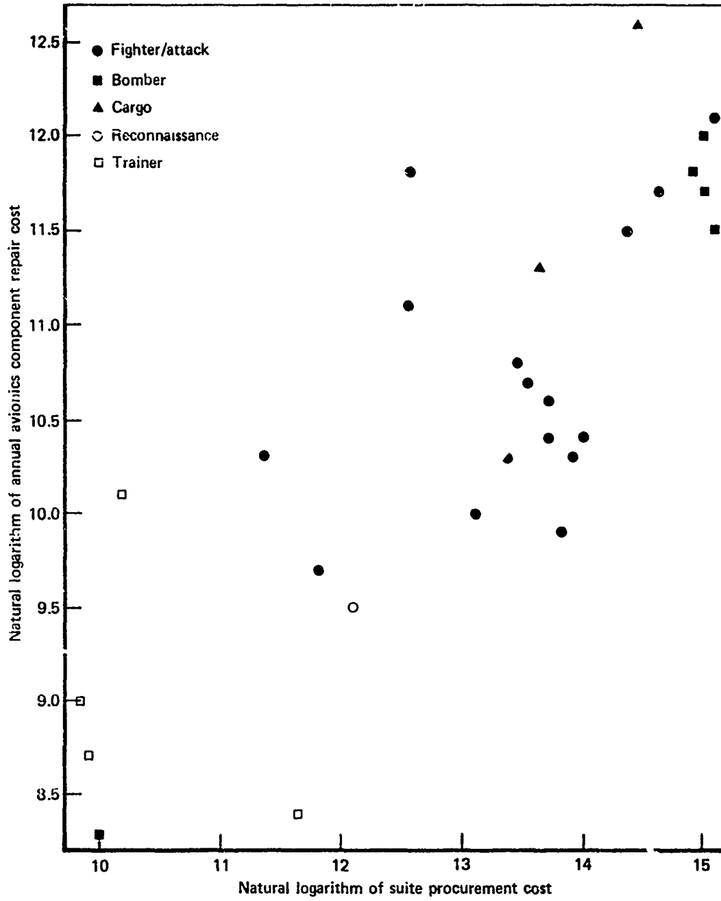
Fig. 8—Variation of annual avionics component repair cost with suite procurement cost
