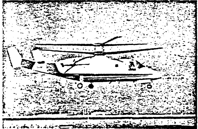
Basic advancing blade concept (ABC) prototype helicopter.
