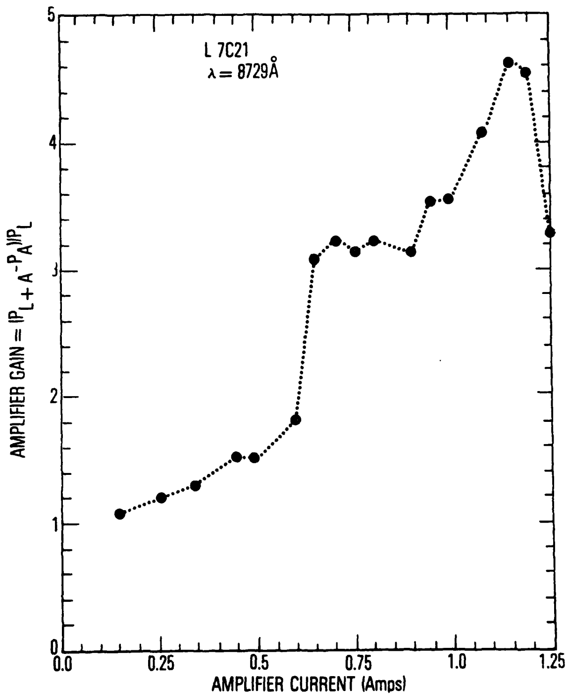
Figure 4. Amplifier gain as a function of amplifier current for diode L7C21 at 8729\text{\AA} .
