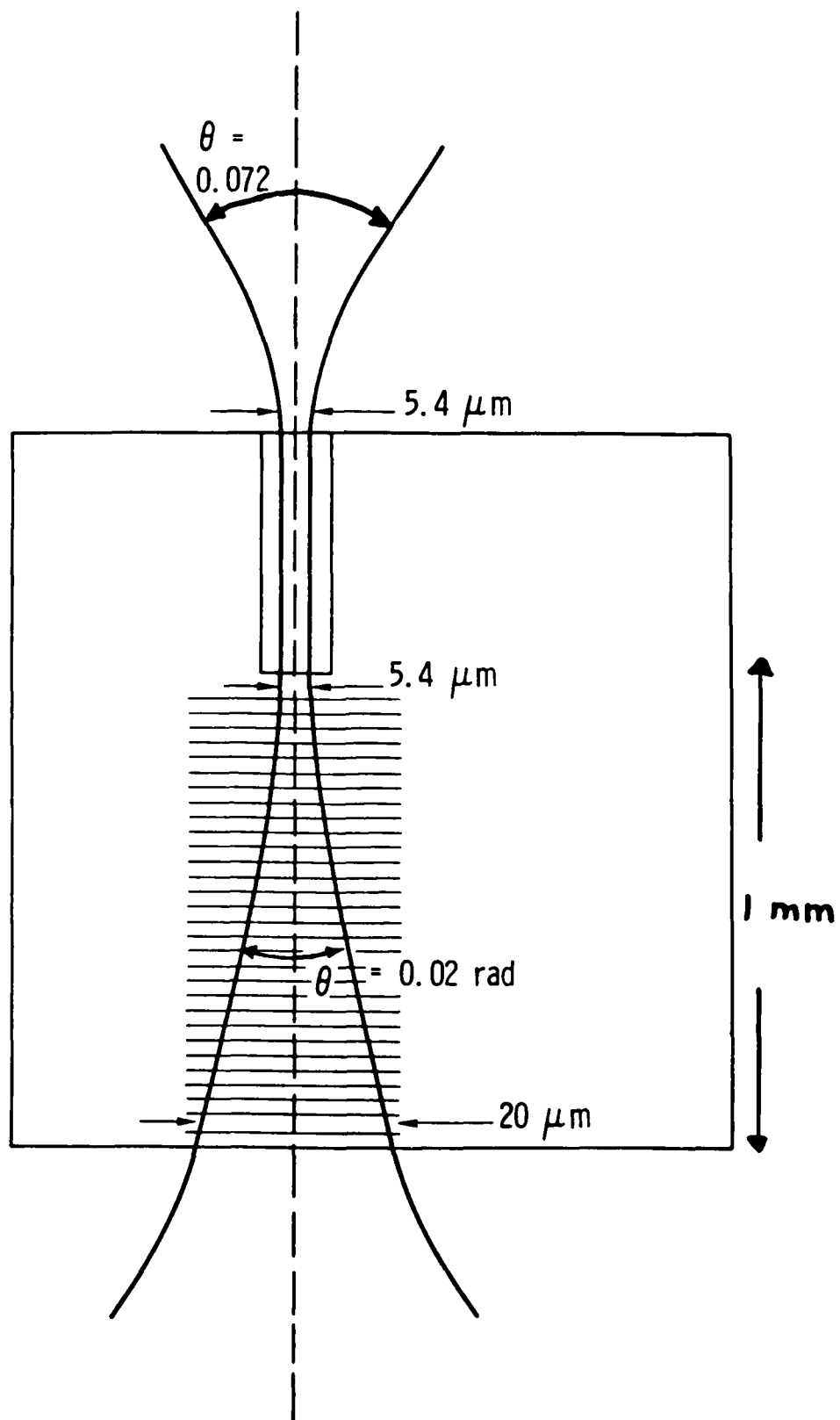
Figure 15 Diagram of top view of DBR laser, showing diffraction limited behavior of diode g9.
