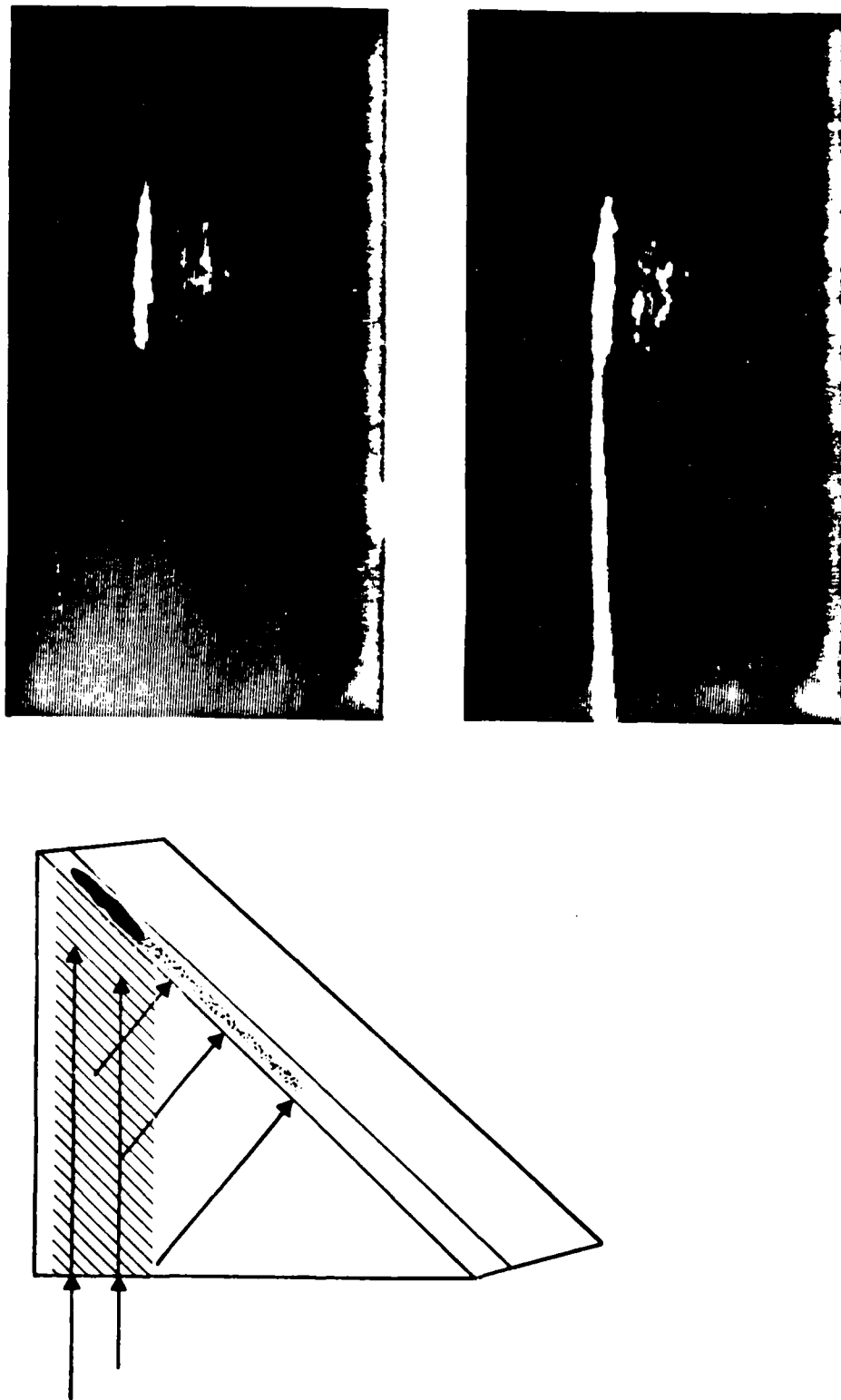
Figure 22 Geometry for 45° beam expander along with photographs of an IR television monitor of near field image of guided beam. The top photograph represents the unexpanded beam 50 \mu\text{m} wide before proper angular alignment. The bottom photograph demonstrates beam expansion with the streak to the left.
