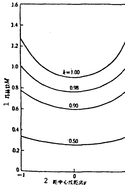
Figure 5. Distribution of Mach number at cross-section of throat n=2.0, r=2.0, \theta_1=23.3^\circ, \gamma=2.0
