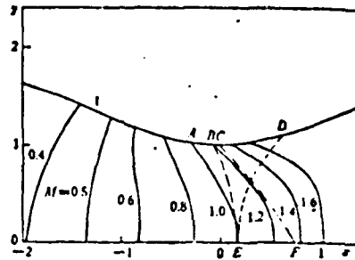
Figure 4. Characteristic lines for supersonic nozzle flow n=2.0, r=2.0, \theta_1=23.3^\circ, \gamma=2.0, k=1.0
