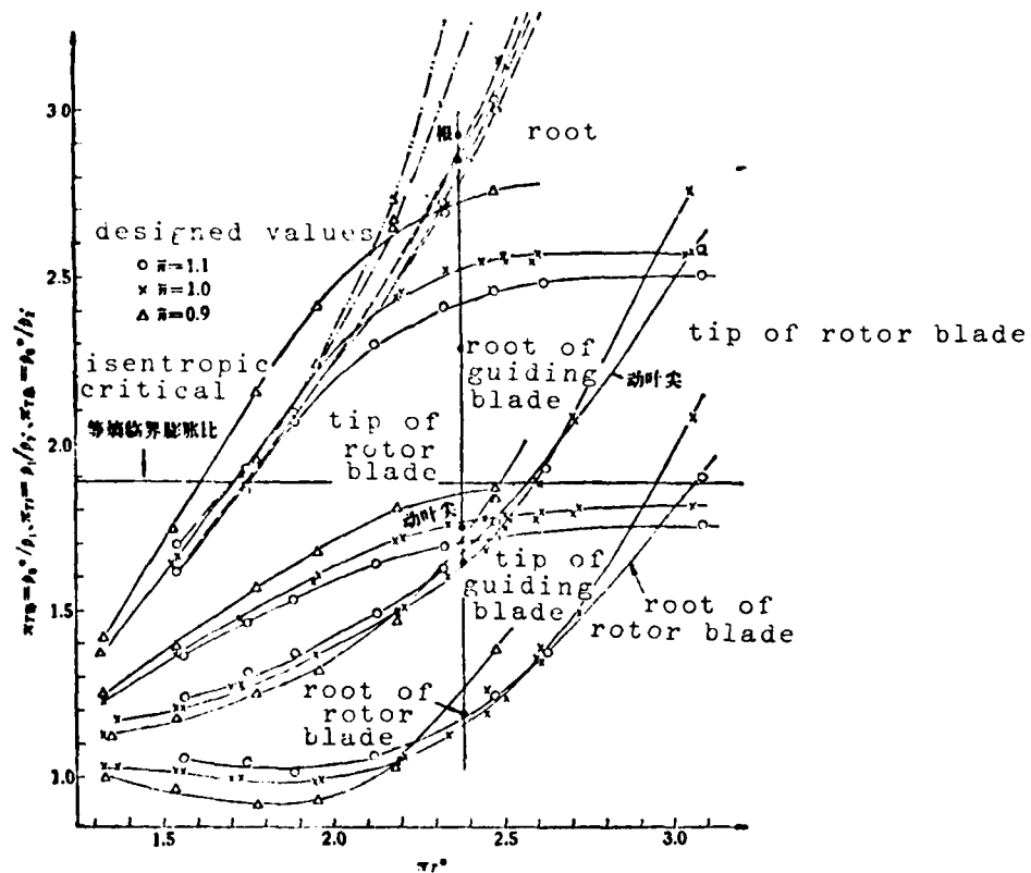
Figure 10. The variation of the expansion ratio vs state
