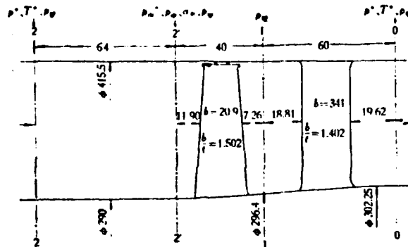
Figure 1. The flow channel and the measuring positions
