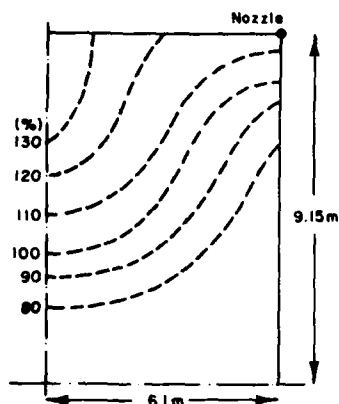
Figure 19. Water distribution contour map.
