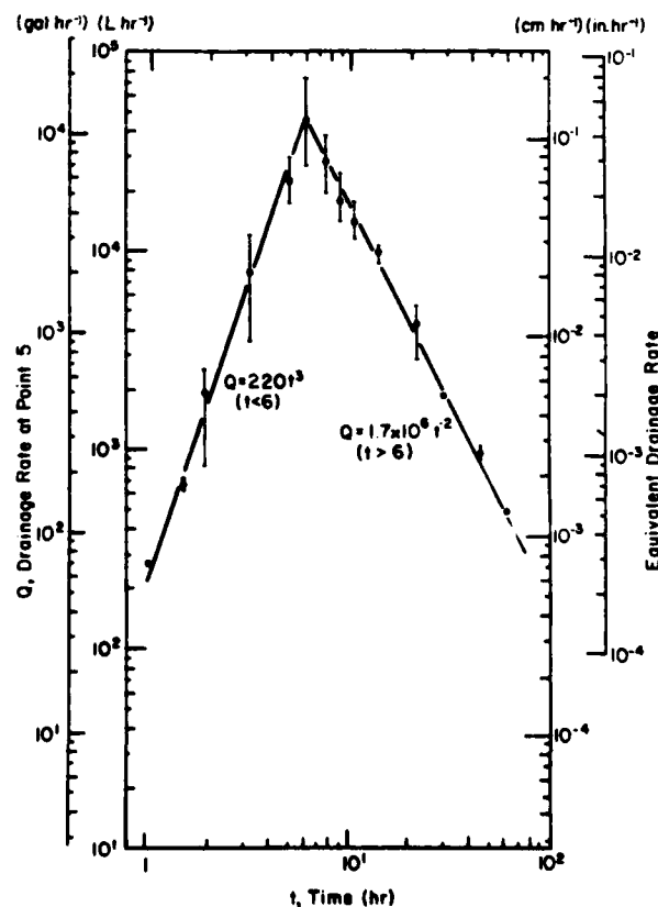
Figure 35. Drainage rate vs time (mean of appl. 3, 5, 8 and 9).
