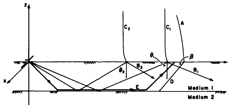
Figure 3. Radiation modes produced by a horizontal electric dipole antenna on the surface of a two-layer ground model. The addition of a second interface has caused wave B of Figure 1 to break into distinct modes (rays B_1, B_2, \dots ) some of which may strongly attenuate with distance. Curves A and D are phase fronts, B_1, B_2 and E are ray normals. C_1 and C_2 indicate amplitude attenuation rates for the surface inhomogeneous waves. Here \beta is the complement of the angle of incidence of phase front D upon the lower interface.
