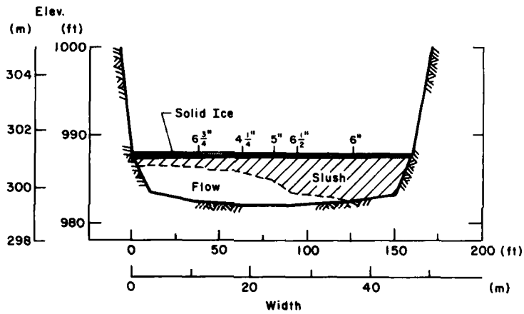
Figure A9. Oil Creek, mile 0.20 (7 February 1980).
