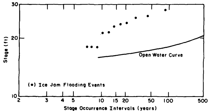
Figure B1. Ice jam floods prior to dredging (11 events in 86 years, 1866-1950).
