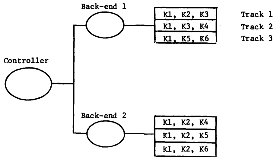
Figure 8a. An Arbitrary Data Placement of 6 Records
