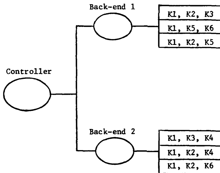
Figure 8b. An Improved Data Placement of Records
