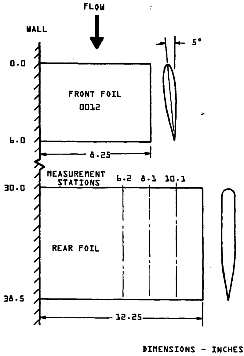
FIGURE 1 - GENERAL CONFIGURATION
