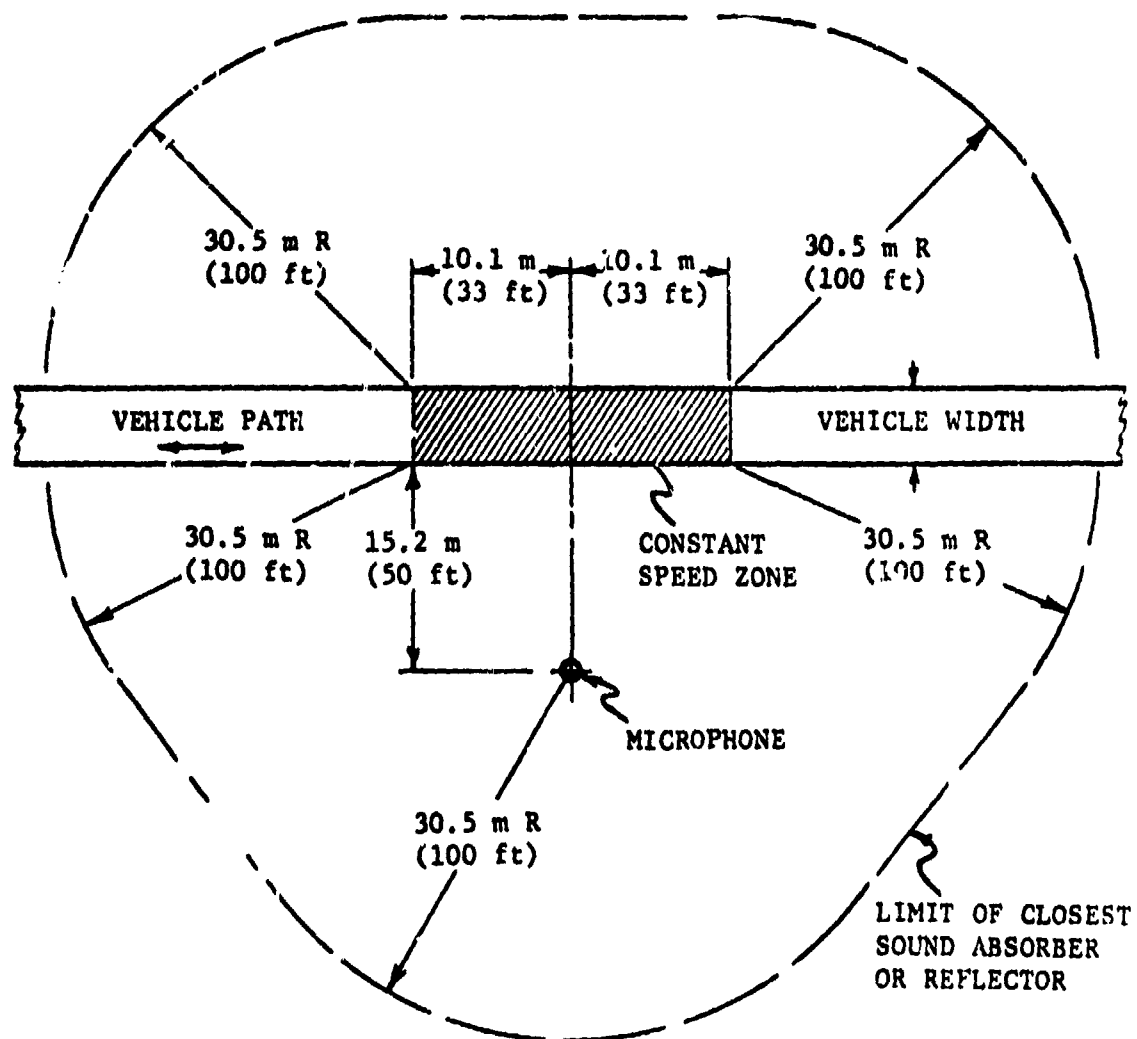
Figure 3. Powered Mobile-Construction-Equipment, Drive-by Noise Test. (From SAE J38a.)
