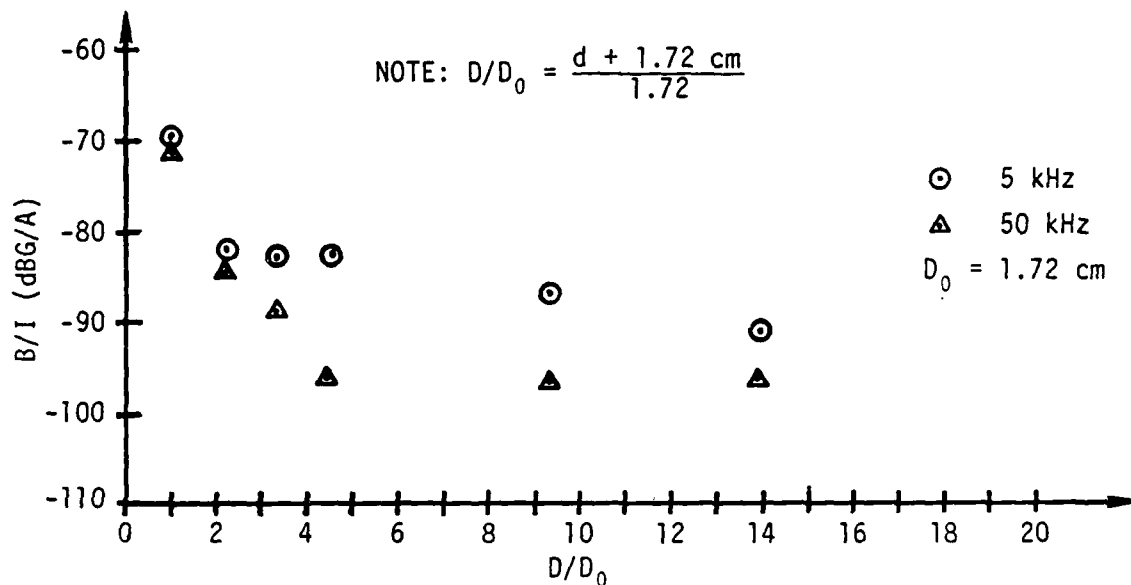
Figure 44a. The Perpendicular Component of Leakage Flux Density in Units of Decibels Relative to 1 Gauss Normalized to 1 A of Primary-Winding Current (B/I) for Frequencies of 5 and 50 kHz. B/I is Shown as a Function of the Probe Spacing Ratio, D/D_0 . The Probe Was Located at the Top Surface of the Jefferson Electric 12438 Transformer Along a Vertical Axis Intersecting the Center of the Seam Nearest the Center of the Case Shown in Figure 3.
