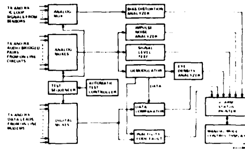
Distortion is measured on each transmit and receive digital circuit by the 'bias/distortion analyzer' as each circuit is multiplexed through the 'analog mux'. Based on data printed out to the controller, appropriate corrective action can be taken. For transmit and receive quasi-analog signals, impulse noise and signal level are measured and the eye pattern of a demodulator connected to the audio bandwidth signal is analyzed for signal levels which exceed threshold levels.
