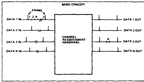
Figure 3. Basic Channel Reassignment Concept
