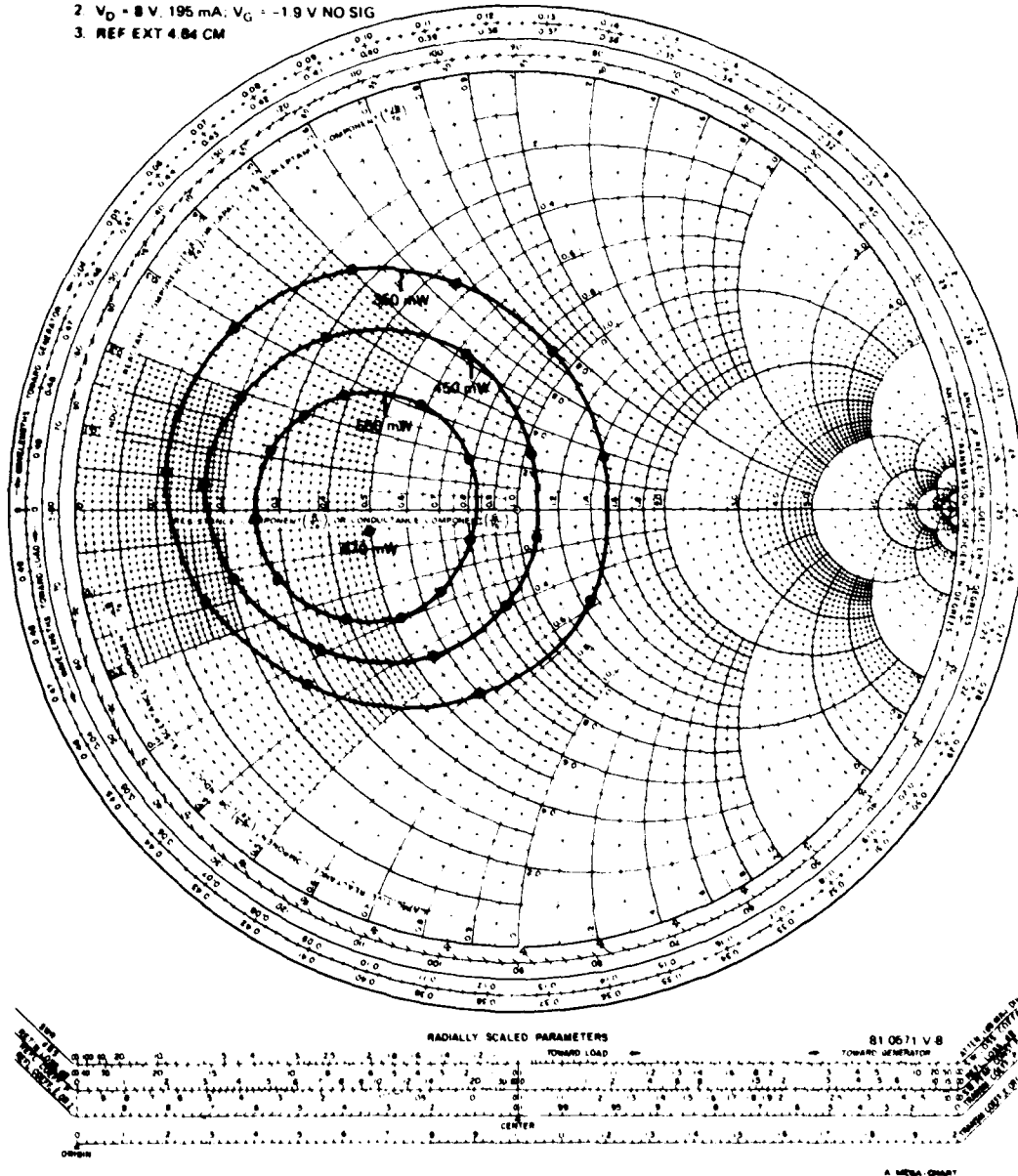
Figure 3-3. Typical Load Pull Data
