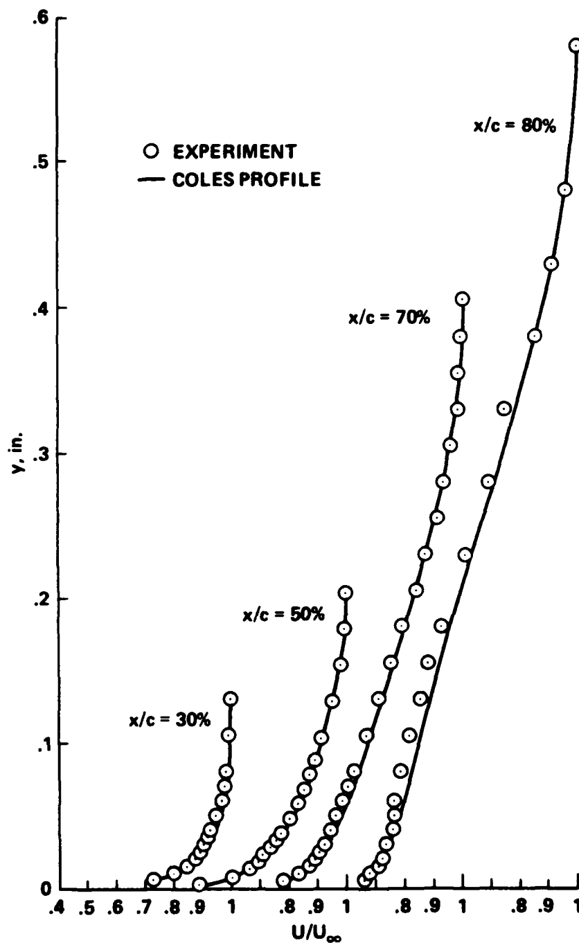
Fig. 11. Time-averaged mean profiles — from Evans
