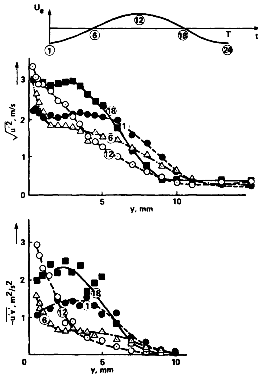
Fig. 13. Profiles of turbulence intensity and Reynolds shear stress — from Cousteix et al. (1977)
