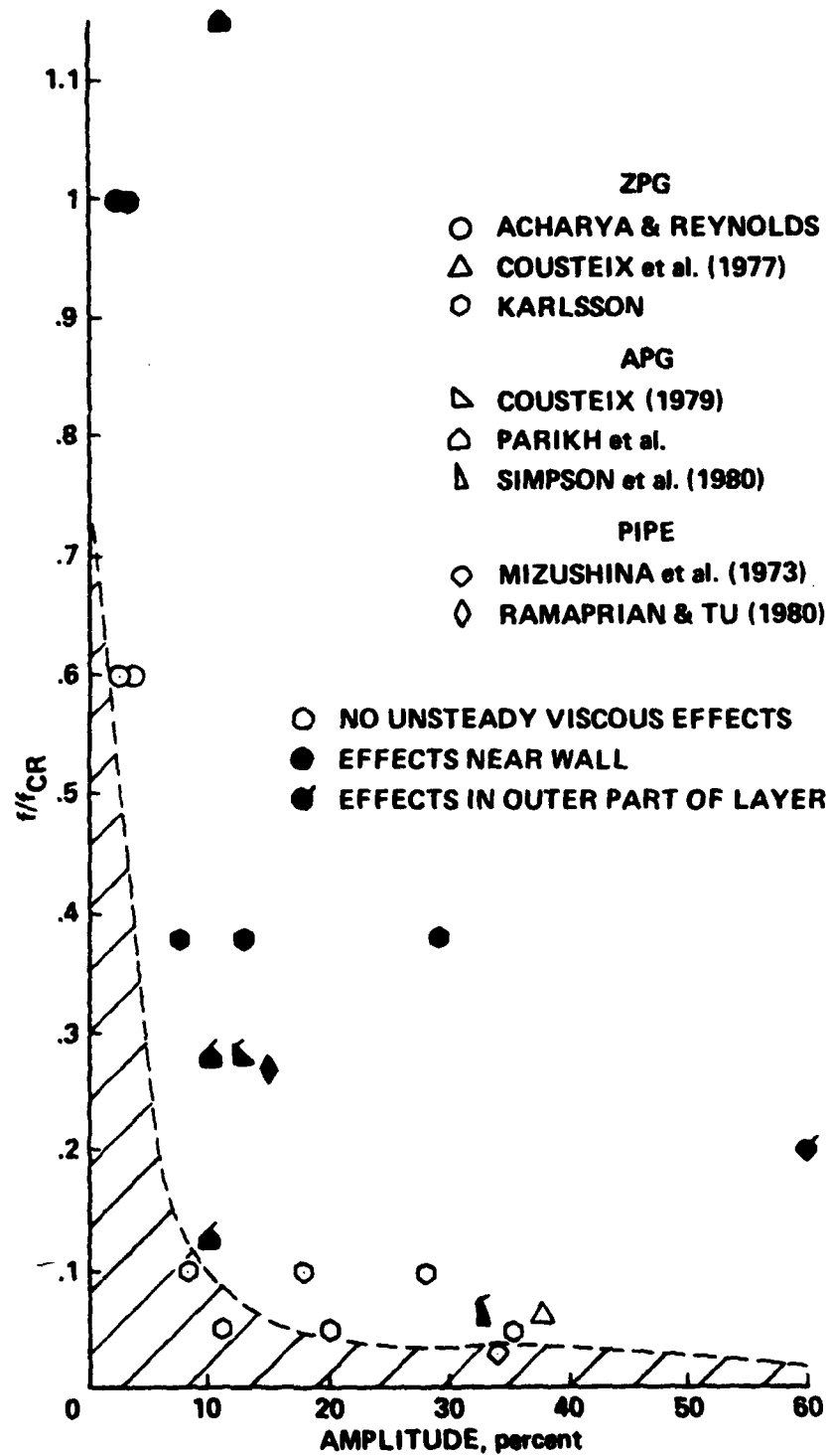
Fig. 20. Ratio of oscillation frequency to turbulent burst frequency for selected experiments
