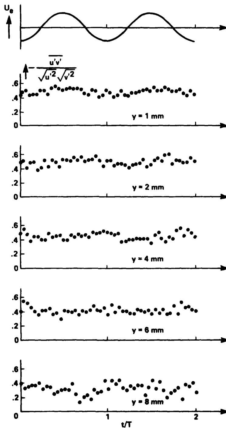
Fig. 14. Statistical distribution of velocity fluctuation — from Cousteix et al. (1977)
