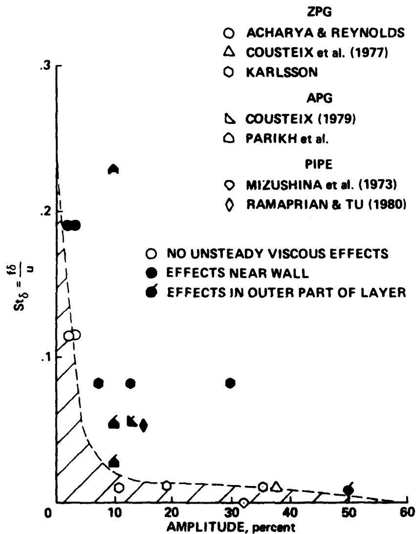
Fig. 19. Strouhal number and amplitude for selected experiments
