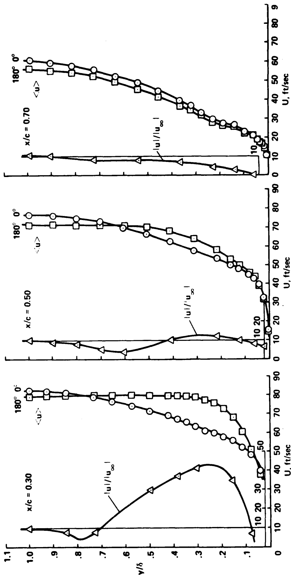
Fig. 12. Ensemble-averaged velocity profiles from Evans
