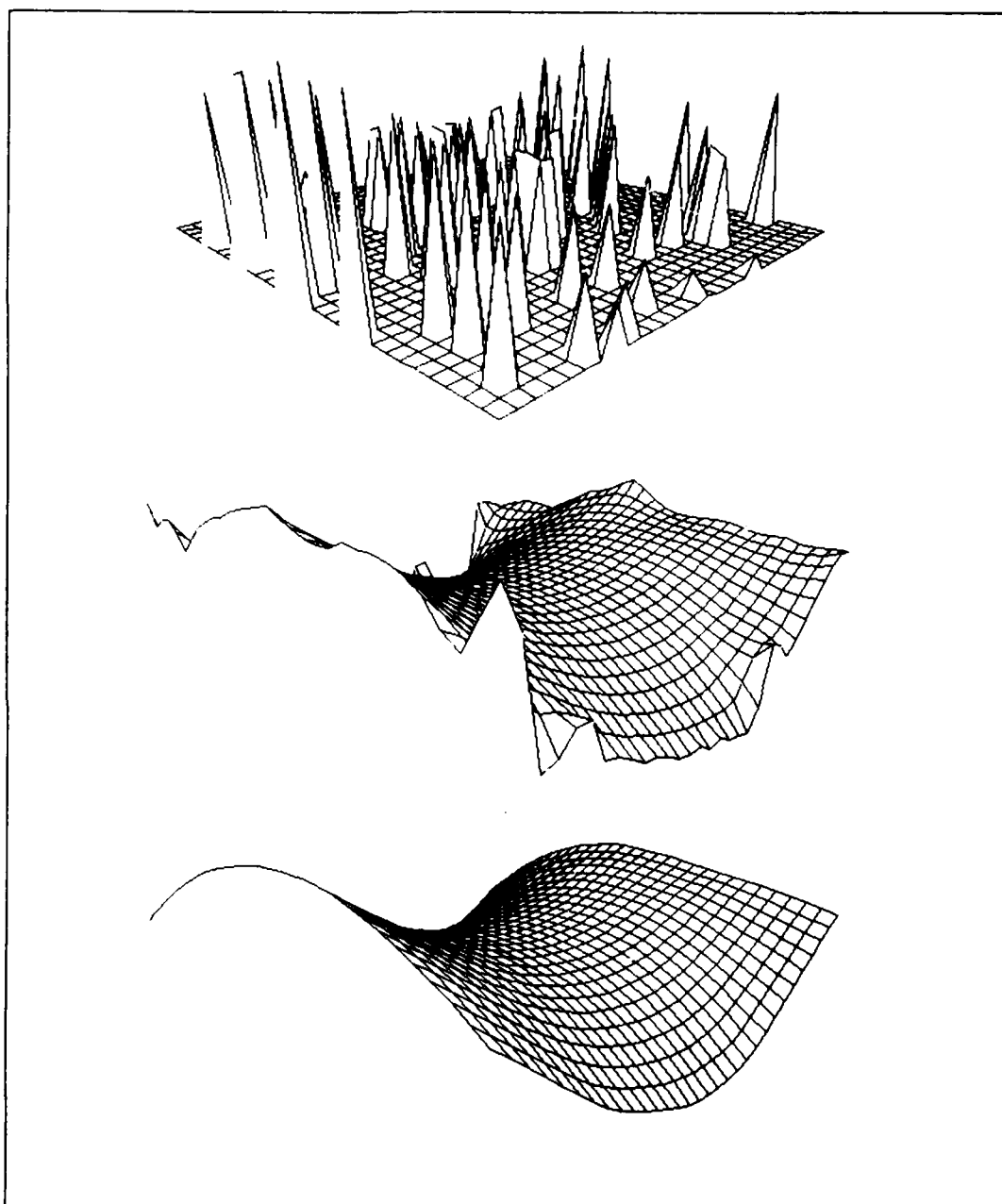
Figure 5. Synthetic Example. The top figure shows a synthetic set of boundary conditions, consistent with a hyperbolic paraboloid. The points are chosen at random with a density of 10 percent. The middle figure shows the surface obtained by applying the gradient projection algorithm to the square Laplacian functional. The bottom figure shows the surface obtained by applying the algorithm to the quadratic variation.
