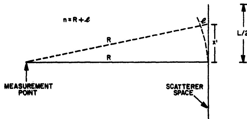
Figure 1. Geometry for Determining Phase Error Due to Finite Measurement Distance
