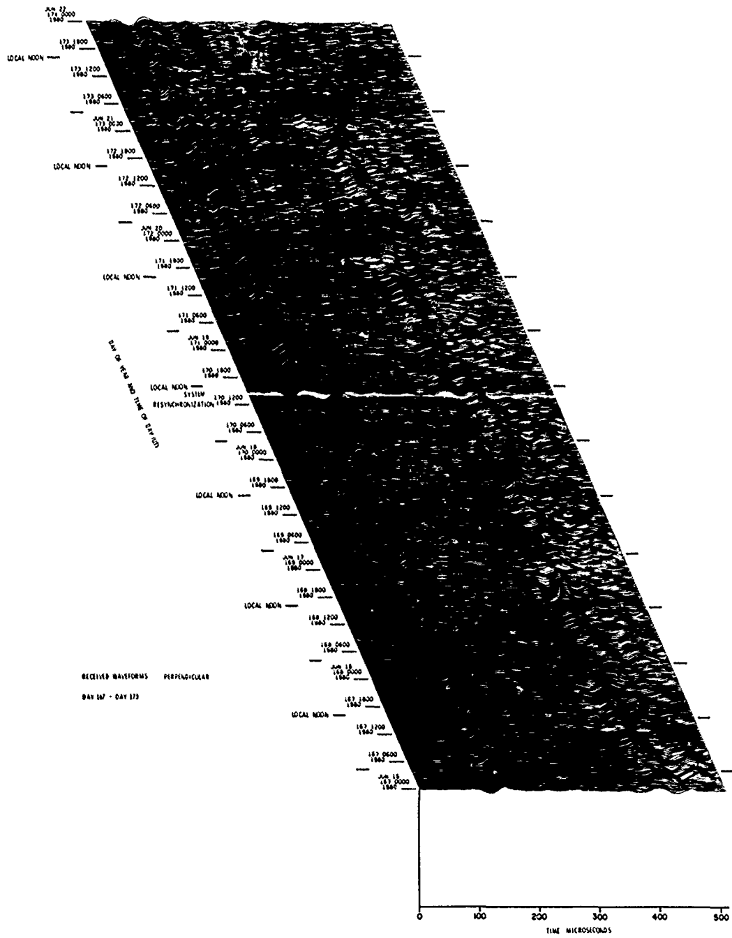
Figure 9. VLF/LF Reflectivity Data for the Polar Ionosphere, DAY 167 (15 Jun) - DAY 173 (21 Jun) 1980 (Cont) Part S. \perp Waveform Display
