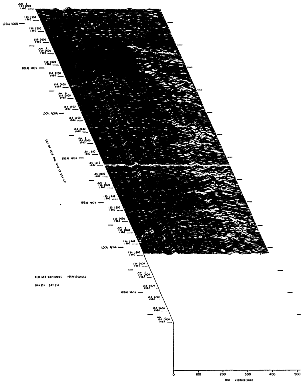
Figure 7. VLF/LF Reflectivity Data for the Polar Ionosphere, DAY 153 (1 Jun) - DAY 159 (7 Jun) 1980 (Cont) Part S. \perp Waveform Display
