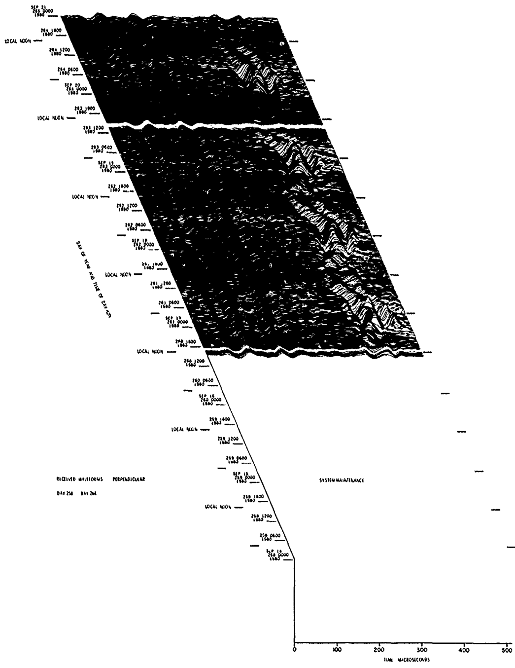
Figure 22. VLF/LF Reflectivity Data for the Polar Ionosphere, DAY 258 (14 Sep) - DAY 264 (20 Sep) 1980 (Cont) Part S. \perp Waveform Display
