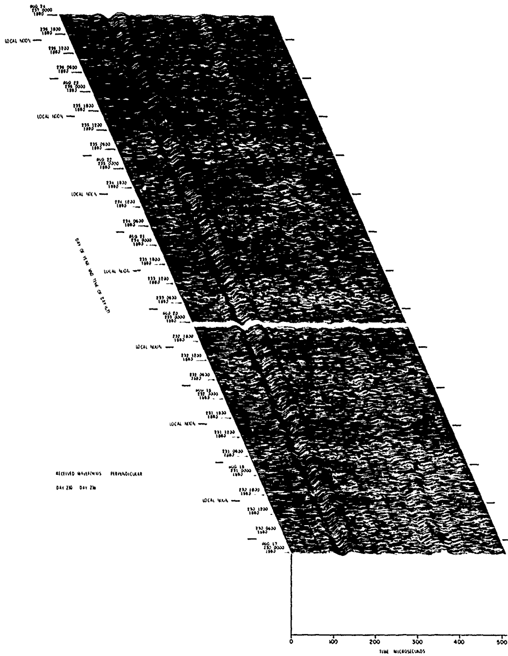
Figure 18. VLF/LF Reflectivity Data for the Polar Ionosphere, DAY 230 (17 Aug) - DAY 236 (23 Aug) 1980 (Cont) Part S. \perp Waveform Display
