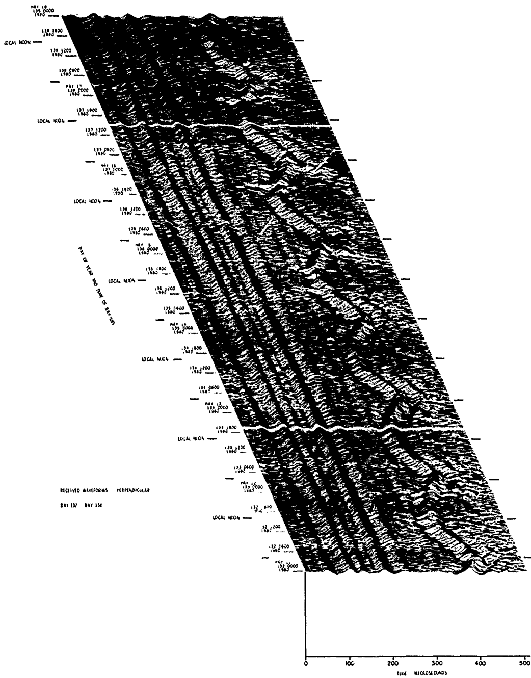
Figure 4. VLF/LF Reflectivity Data for the Polar Ionosphere, DAY 132 (11 May) - DAY 138 (17 May) 1980 (Cont) Part S. \perp Waveform Display
