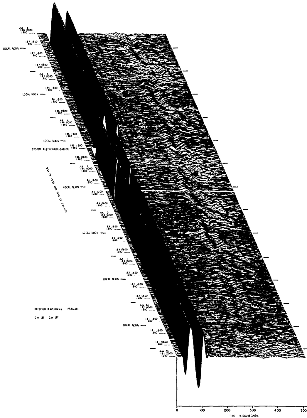
Figure 11. VLF/LF Reflectivity Data for the Polar Ionosphere, DAY 181 (29 Jun) – DAY 187 (5 Jul) 1980 (Cont) Part R. || Waveform Display
