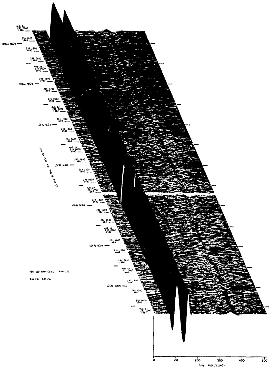
Figure 18. VLF/LF Reflectivity Data for the Polar Ionosphere, DAY 230 (17 Aug) - DAY 236 (23 Aug) 1980 (Cont) Part R. || Waveform Display
