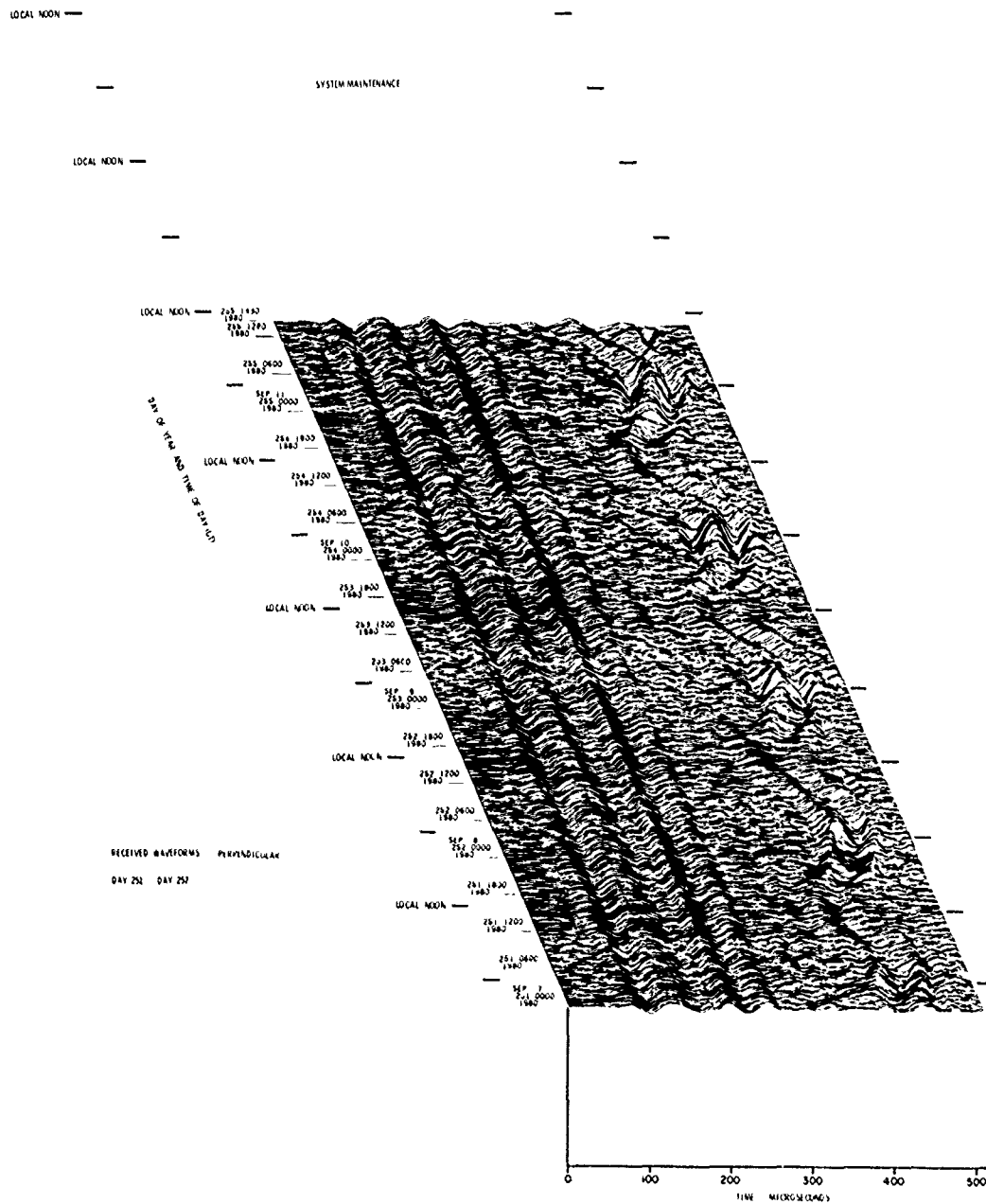
Figure 21. VLF/LF Reflectivity Data for the Polar Ionosphere, DAY 251 (7 Sep) – DAY 257 (13 Sep) 1980 (Cont) Part S. \perp Waveform Display
