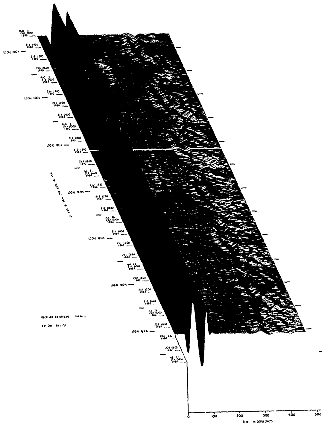
Figure 15. VLF/LF Reflectivity Data for the Polar Ionosphere, DAY 209 (27 Jul) - DAY 215 (2 Aug) 1980 (Cont) Part R. || Waveform Display
