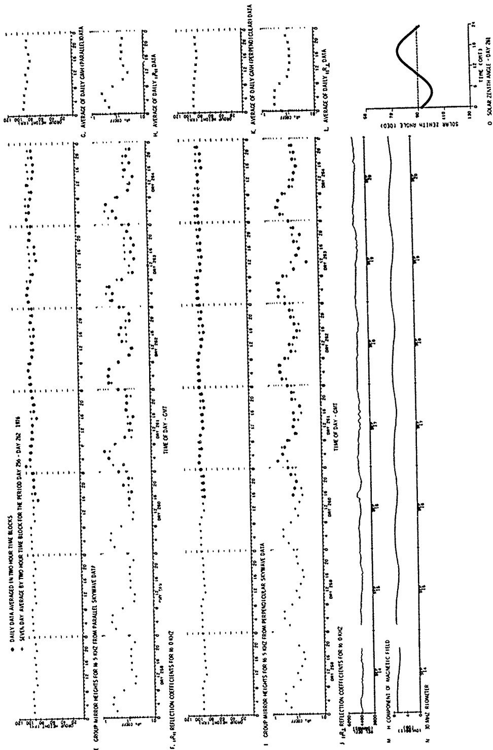
Figure 22. VLF/LF Reflectivity Data for the Polar Ionosphere, DAY 258 (14 Sep) - DAY 264 (20 Sep) 1980 (Cont)
