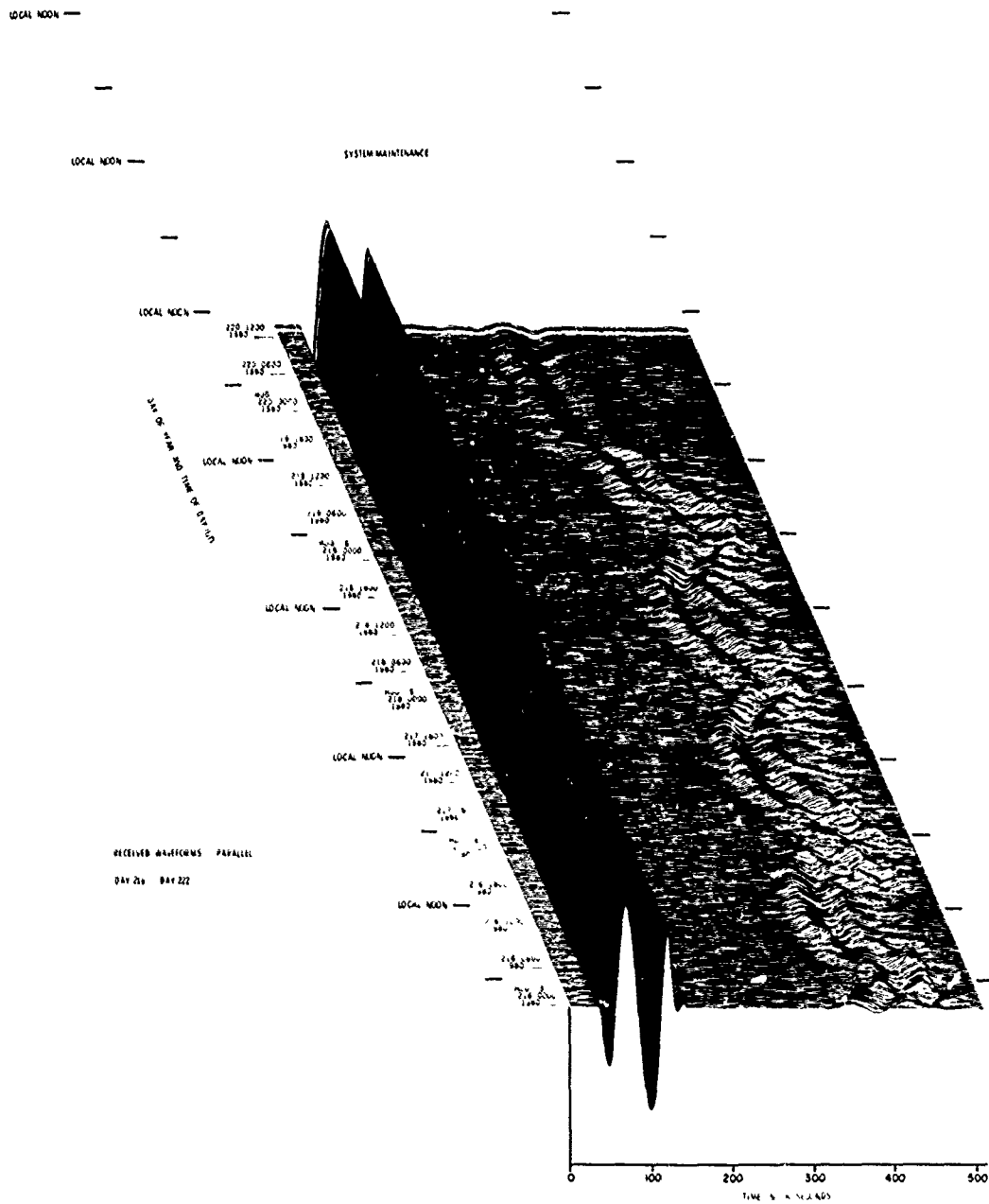
Figure 16. VLF/LF Reflectivity Data for the Polar Ionosphere, DAY 216 (3 Aug) - DAY 222 (9 Aug) 1980 (Cont) Part R. || Waveform Display
