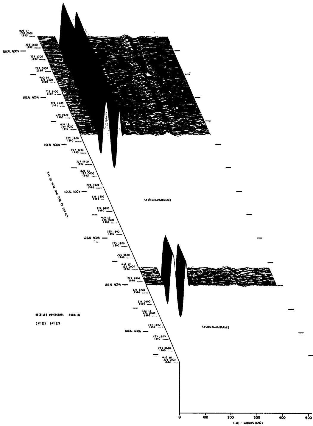
Figure 17. VLF/LF Reflectivity Data for the Polar Ionosphere, DAY 223 (10 Aug) - DAY 229 (16 Aug) 1980 (Cont) Part R. || Waveform Display
