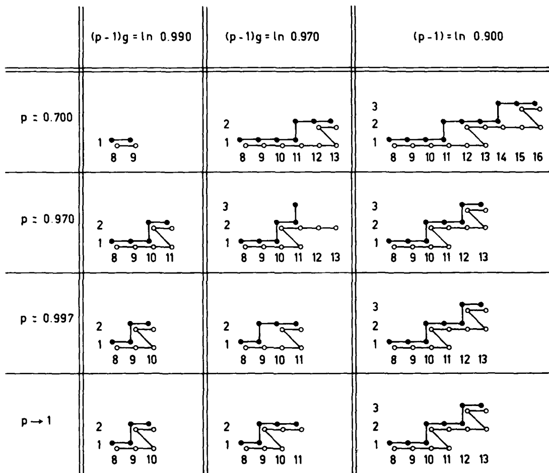
FIGURE 5. Allocation sequences optimizing R_{ap}
