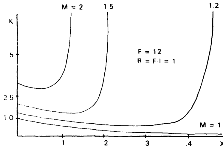
FIGURE 2. The optimal value of K as a function for a range of M values
