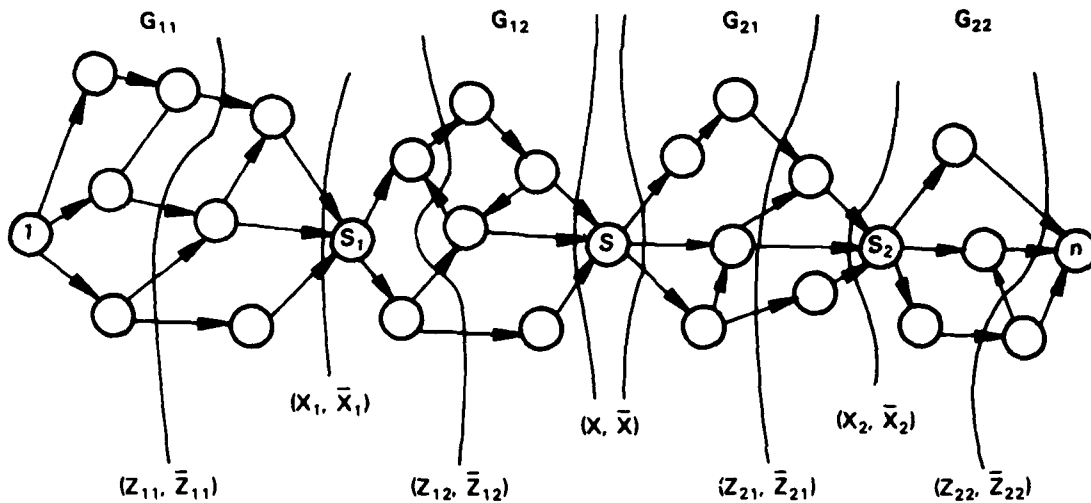
FIGURE 2. G_1 and G_2 are further decomposed into G_{11} , G_{12} , and G_{21} , G_{22} .
