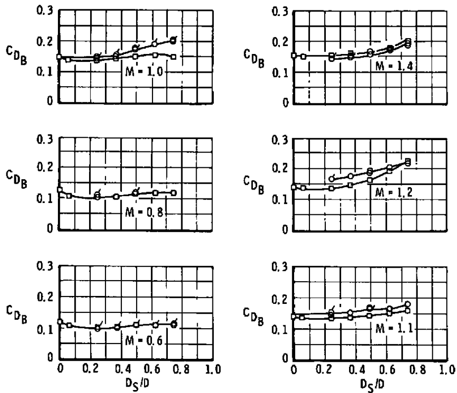
Figure 5. Base drag as a function of sting diameter ratio [4].
