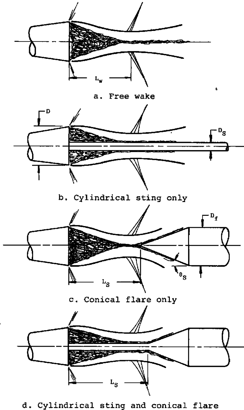
Figure 3. Combinations of cylindrical sting and conical flare interference configurations.
