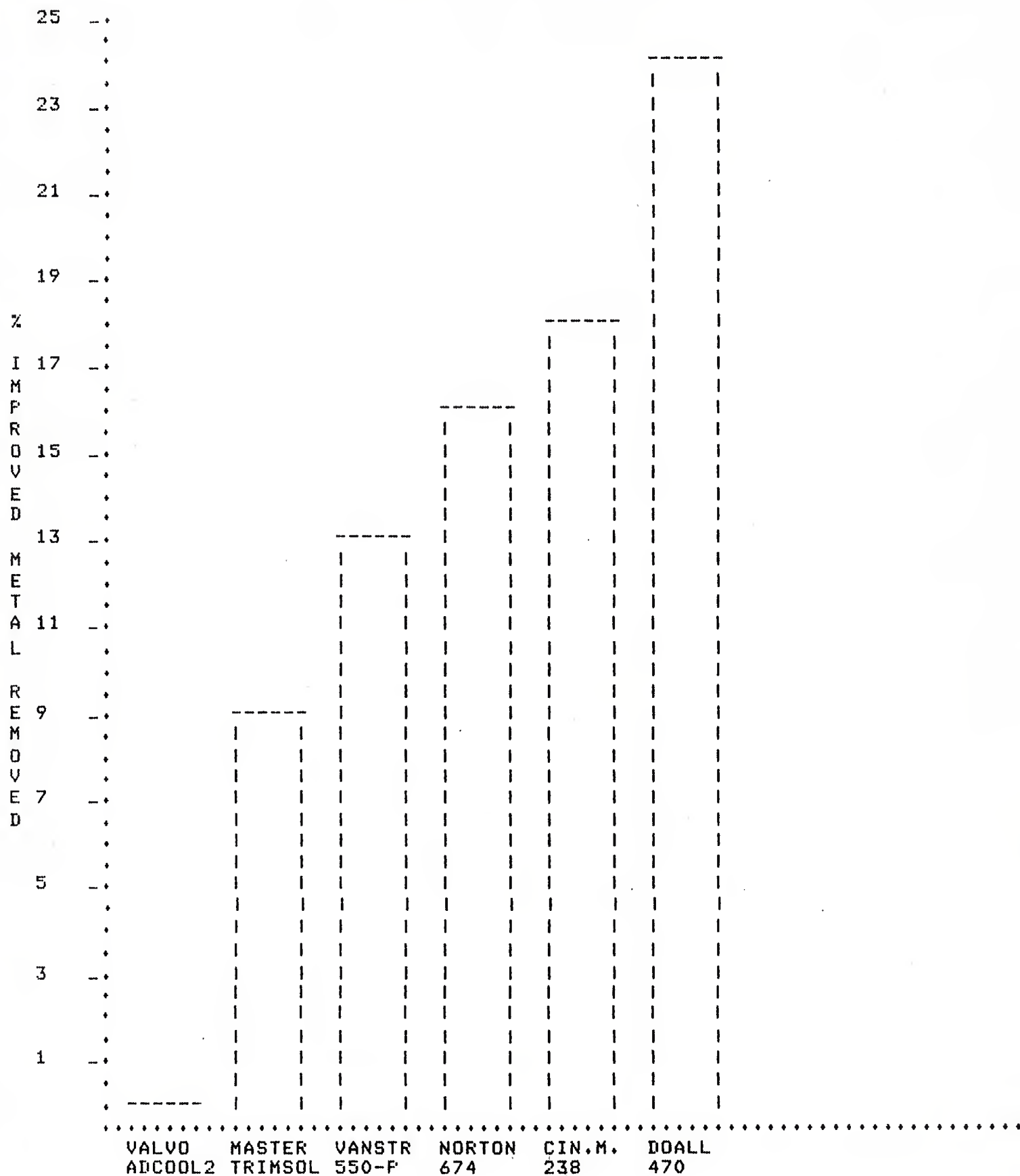
Figure 3.6-7. Percent Improved Tool Life Compared to Adcool-2.
