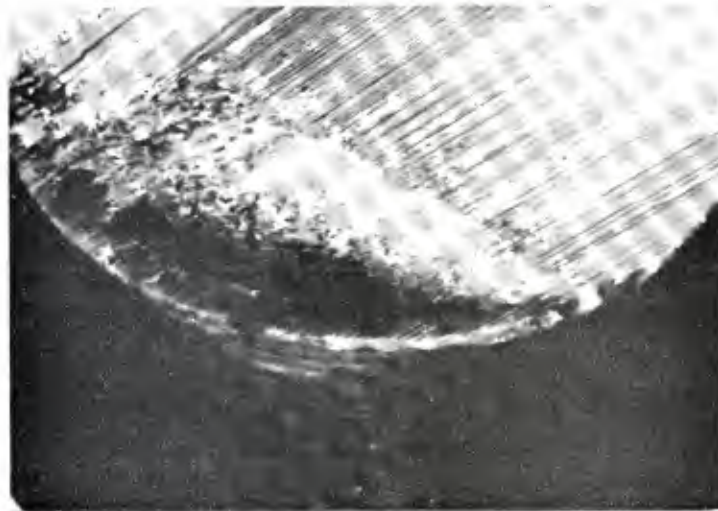
b) AFTER ANALYSIS - GRADUAL CRATER WEAR
