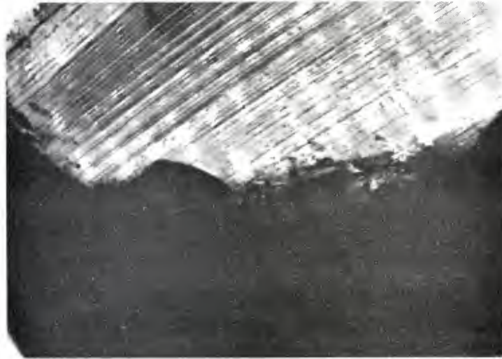
a) ORIGINAL WEAR - CHIPPING AND WELDING
