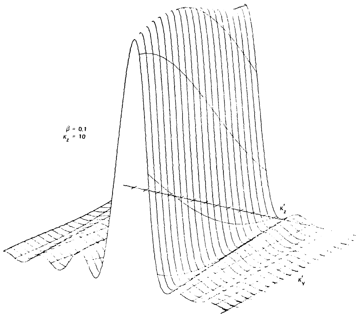
FIGURE 2 PERSPECTIVE PLOT SHOWING 1/L|D_L|^2 AS A FUNCTION OF k'_Y AND k'_Z FOR SMALL \beta AND LARGE \kappa_Z
