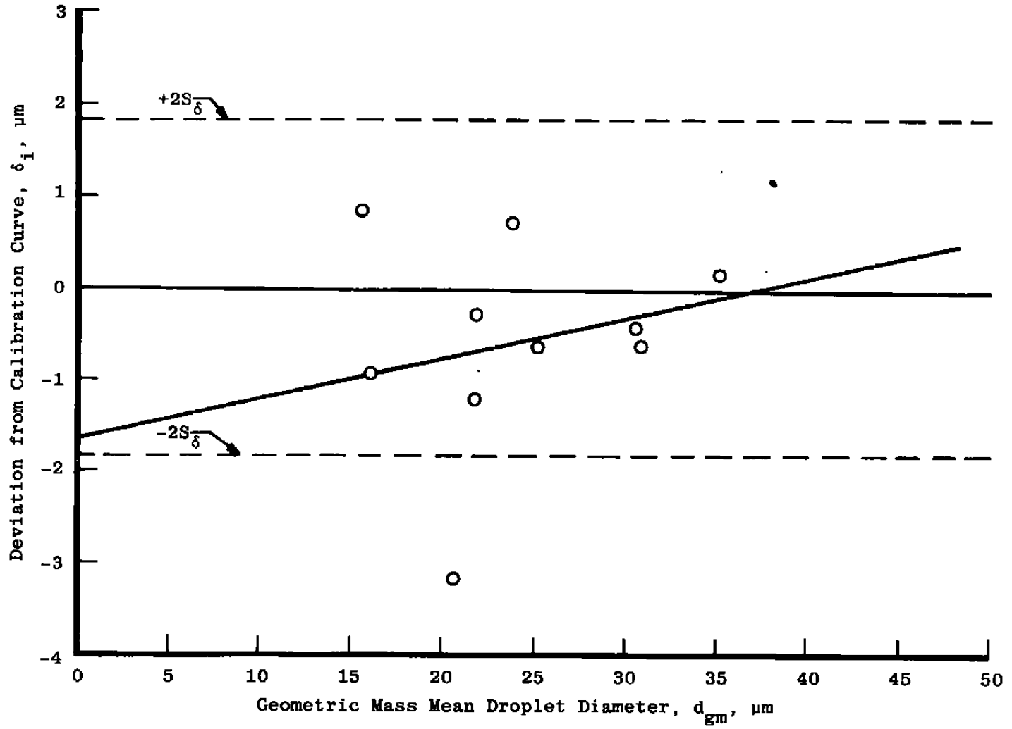
Figure 31. Deviation of FOS data from holographic calibration data.
