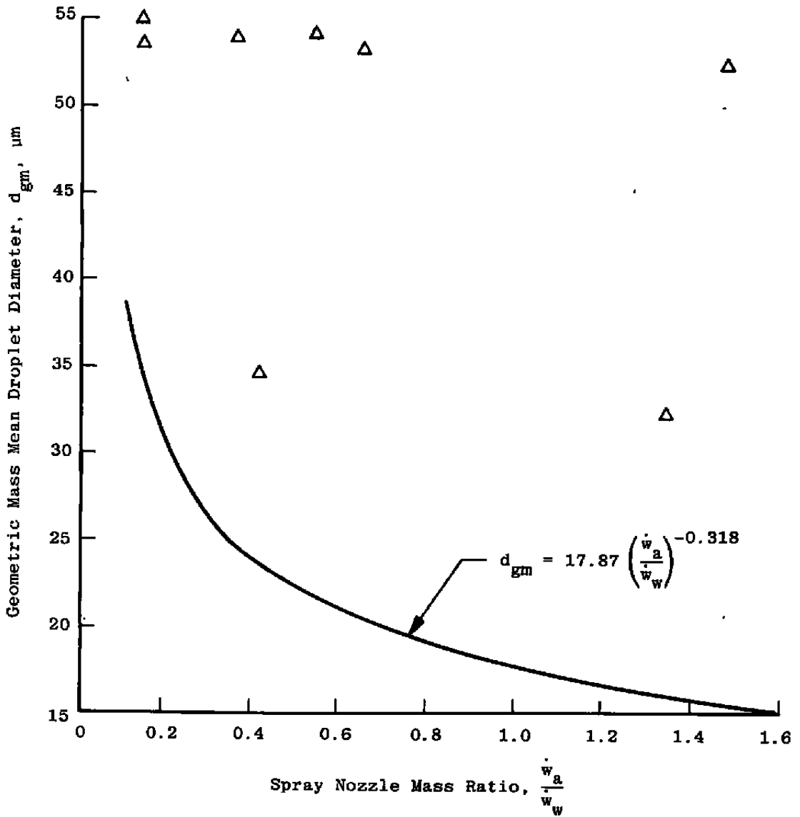
Figure 38. Comparison of commercial-PSI data with spray nozzle calibration.
