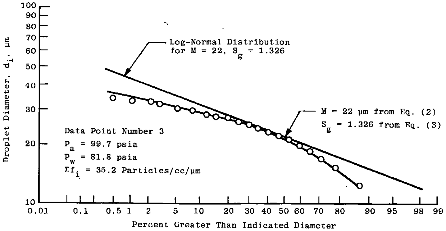
Figure 33. Typical log-probability plot for AEDC-PSI.
