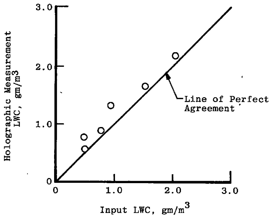
Figure 26. Calculated LWC vs input LWC.
