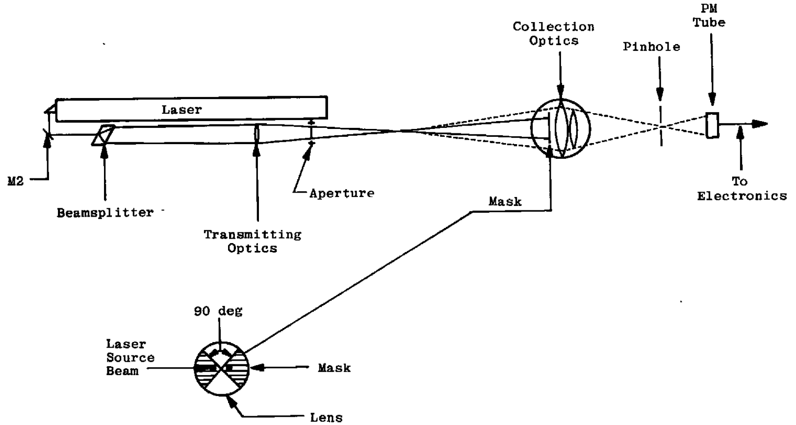
Figure 13. Commercial-PSI optical system.
