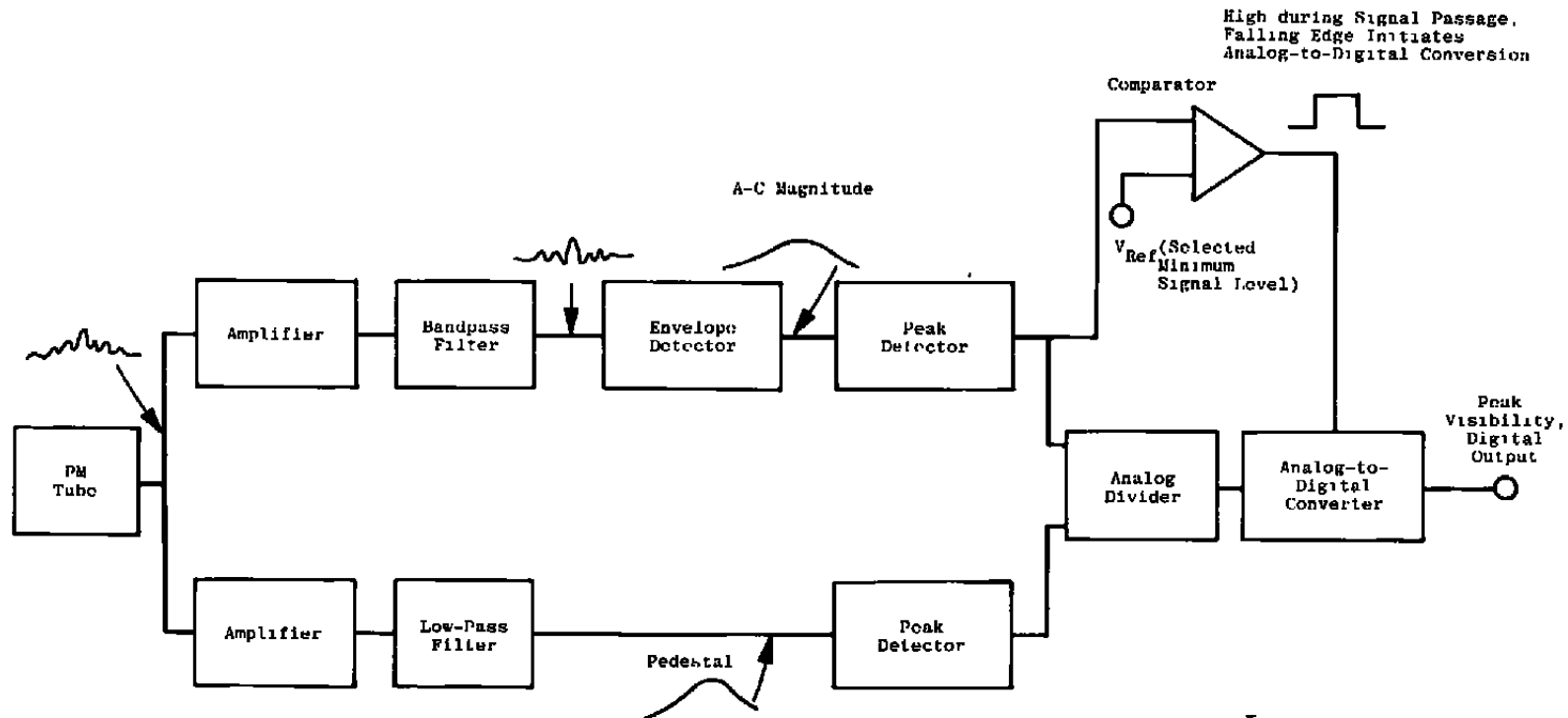
Figure 12. Electronics for AEDC-developed PSI.
