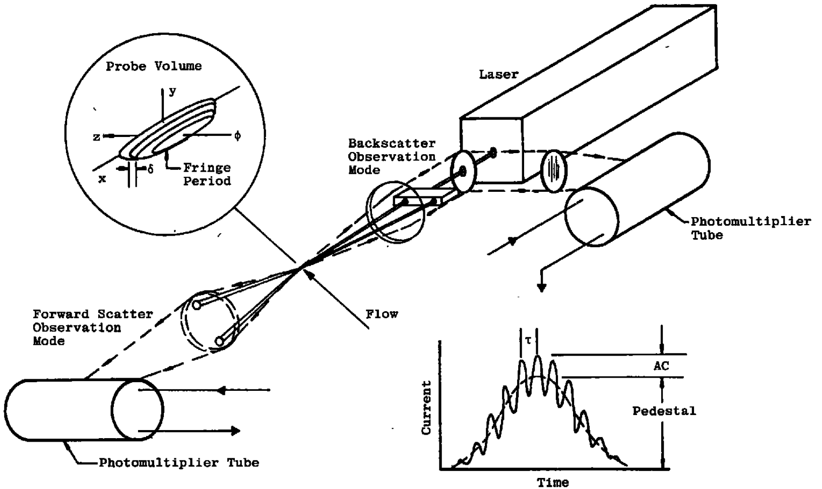
Figure 10. Particle-sizing interferometer.
