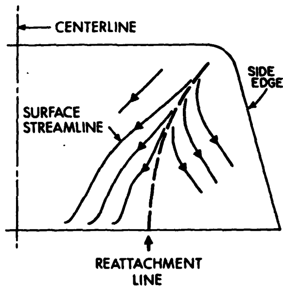
Figure 4. Rear View of a Slanted Base Showing Part of the Surface Flow Pattern. The Flow along the Side (Out of the Plane of the Paper) Separates at the Side Edge and Reattaches at the Dashed Line. Sketched from a Photograph in (3)
