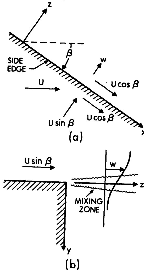
Figure 6. Flow Over an Infinite, Yawed Side Edge at y = 0 , z = 0
