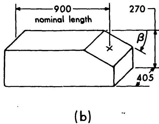
Figure 1. Models Tested by Morel (2). Dimensions in mm.
