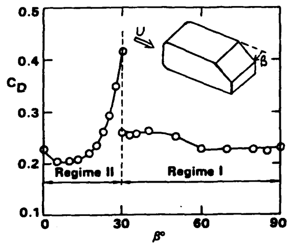
Figure 2. Drag Coefficient of the Vehicle-Like Model in the Free Stream Location, From (2)
