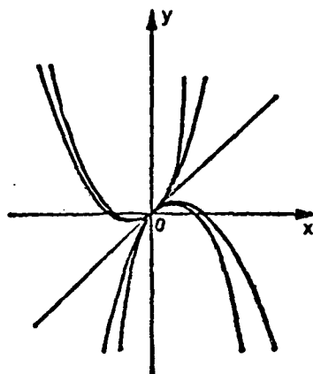
Figure 11. Quasiradial orbits
