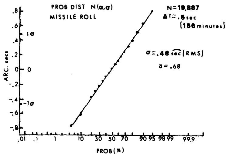
Fig 2 - HETF Missile Distribution in Roll Over 166 min Benign Environment
