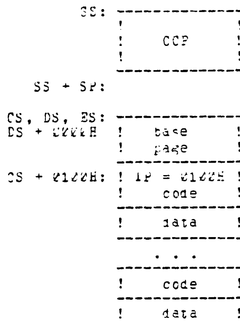
Figure 2 The BCB Memory Model.
