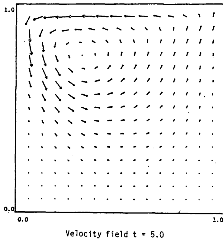
Figure 5.7 Discrete solution of the time dependent Navier Stokes equation at Reynold's number 200.
