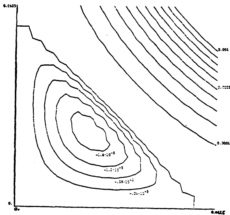
Figure 5.3 Contour plots of the first biharmonic eigenfunction near a corner.
