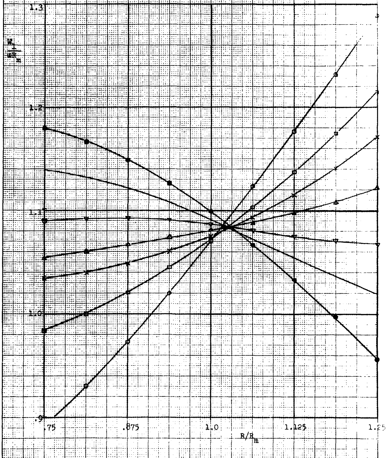
FIG. 6 DISTRIBUTION OF THE RELATIVE VELOCITY AHEAD OF THE ROTOR ( \xi = 0 ) (Symbols, see Fig. 4)
