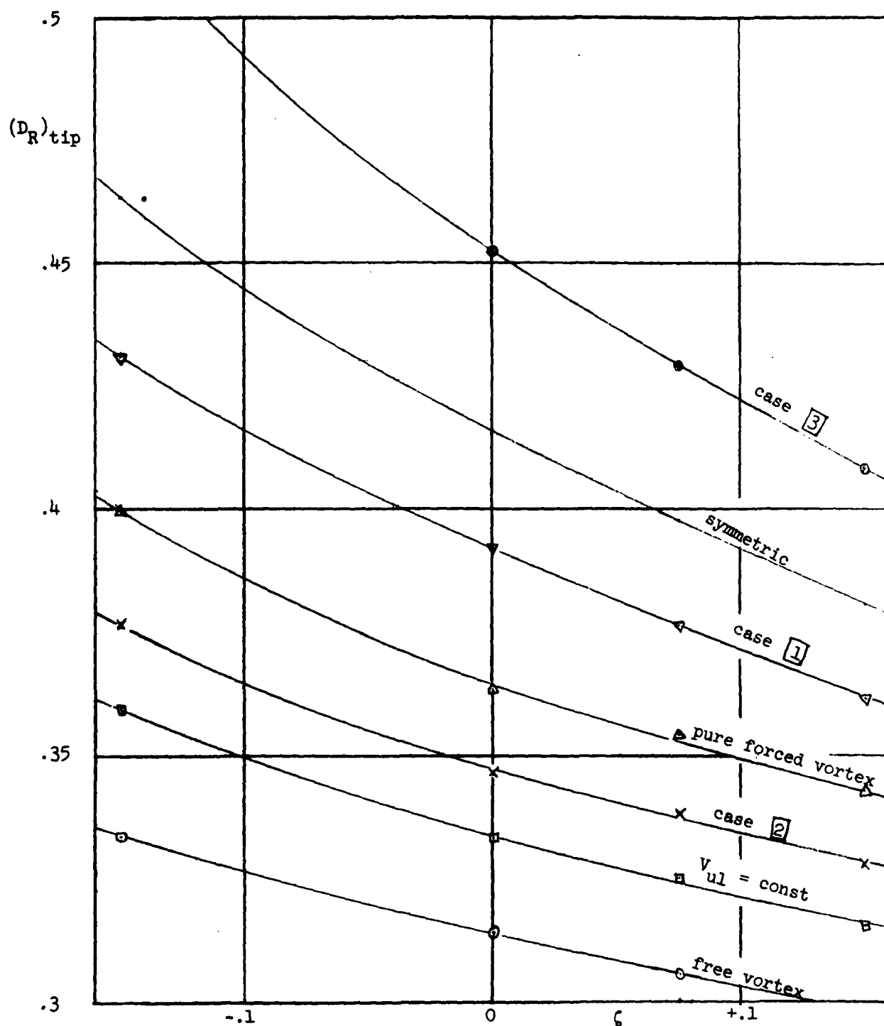
FIG. 14 INFLUENCE OF IMPOSED ENTHALPY GRADIENT ON THE NACA DIFFUSION FACTOR AT ROTOR TIP
